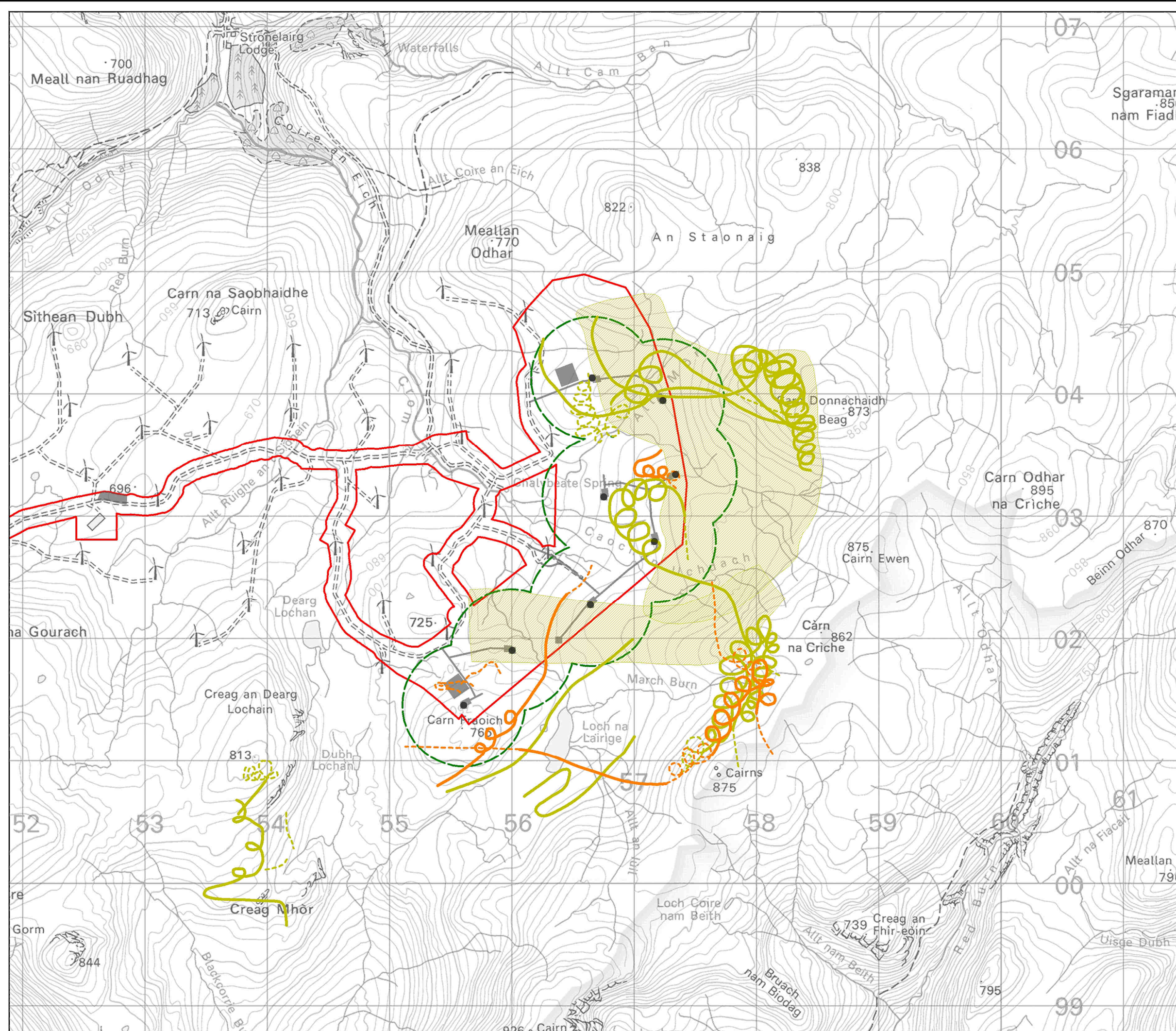
Figure 9.6b Flight Activity by Golden Eagle (Feb-Aug 2019, Eastern Cluster) Cloiche Wind Farm EIA Report
