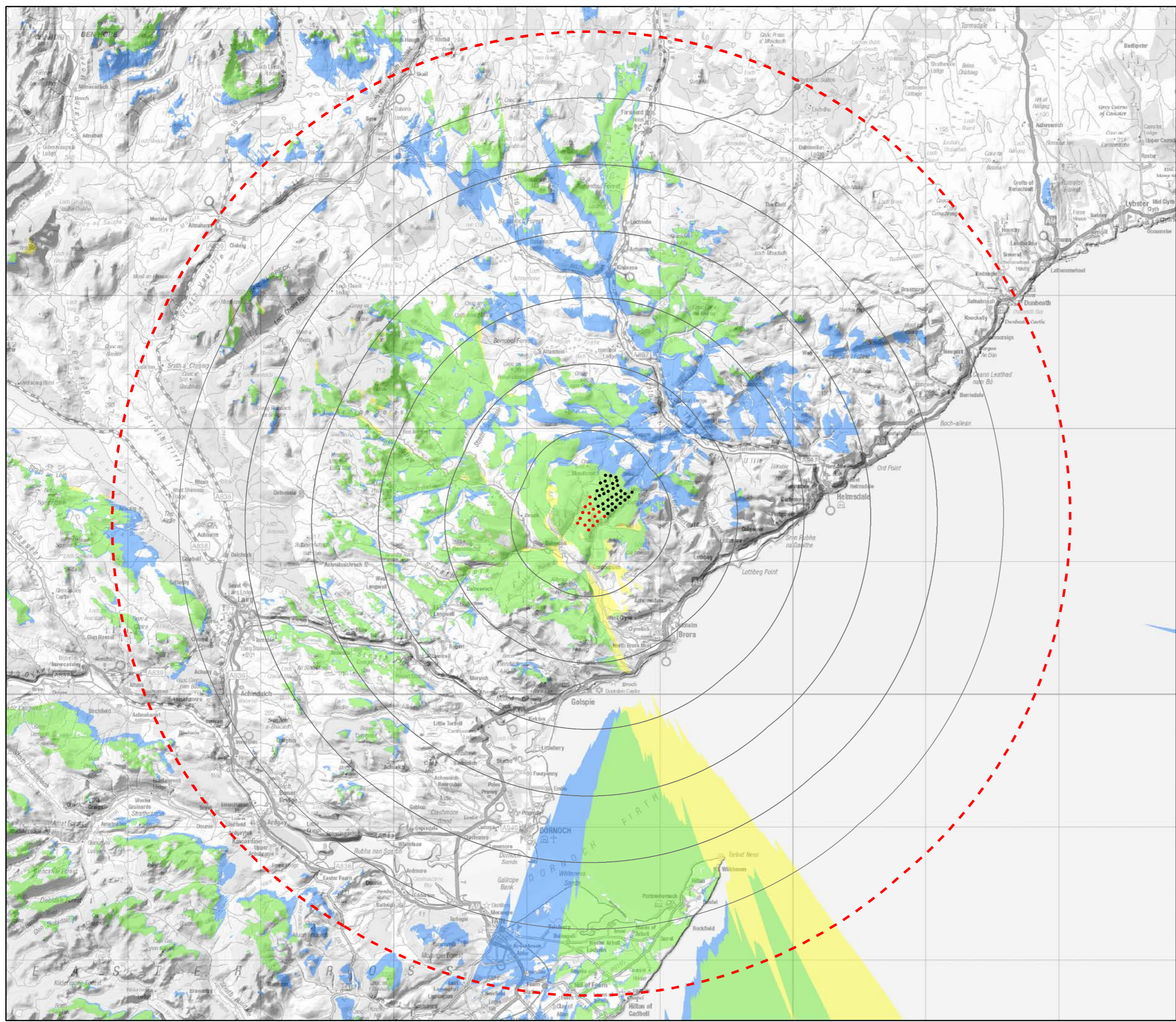
Figure 7.16d CUMULATIVE ZTV WITH GORDONBUSH Gordonbush Extension Wind Farm Environmental Statement
