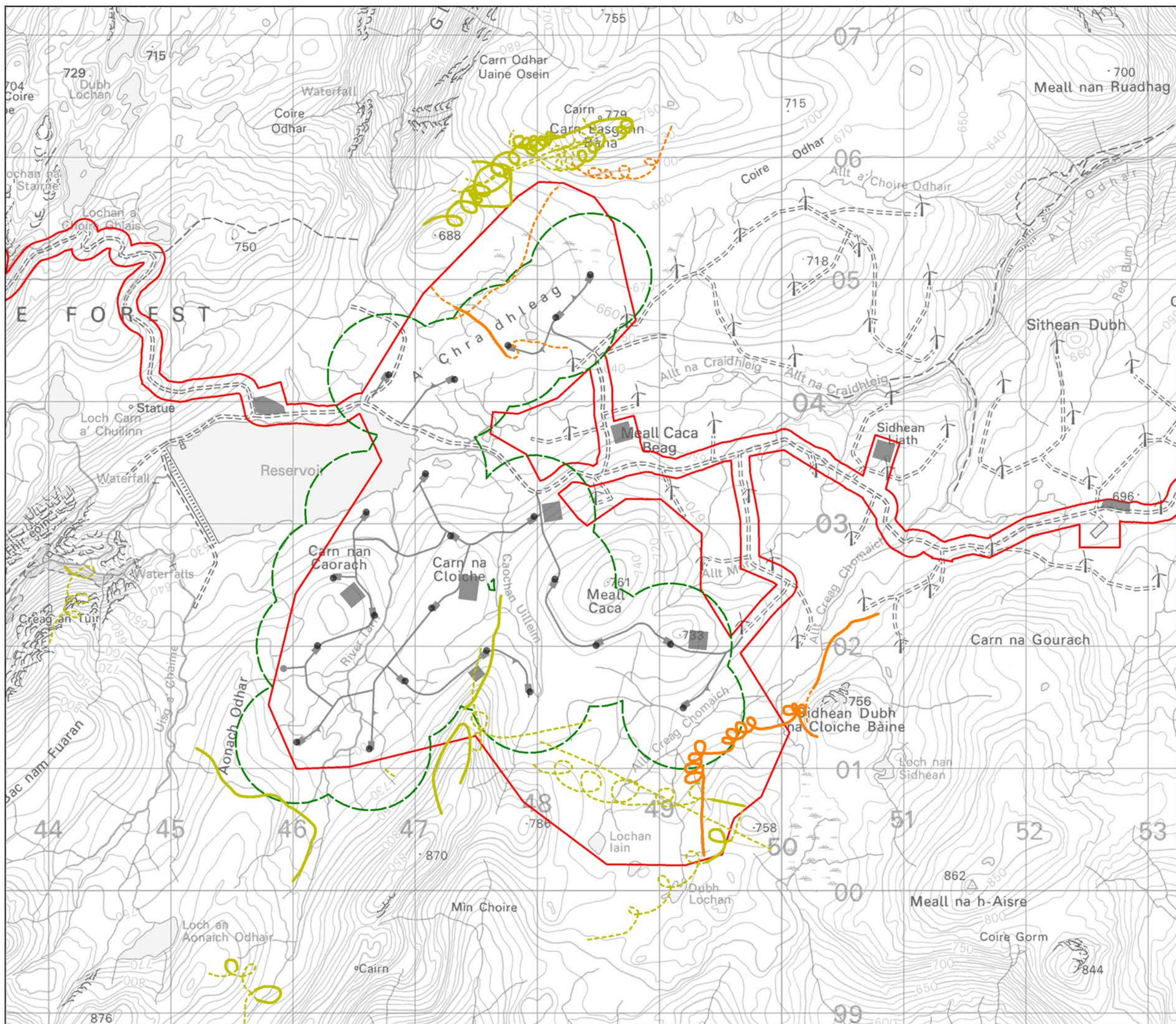
Figure 5.6a Flight Activity by Golden Eagle (Feb-Aug 2019, Western Cluster) Cloiche Wind Farm Additional Information
