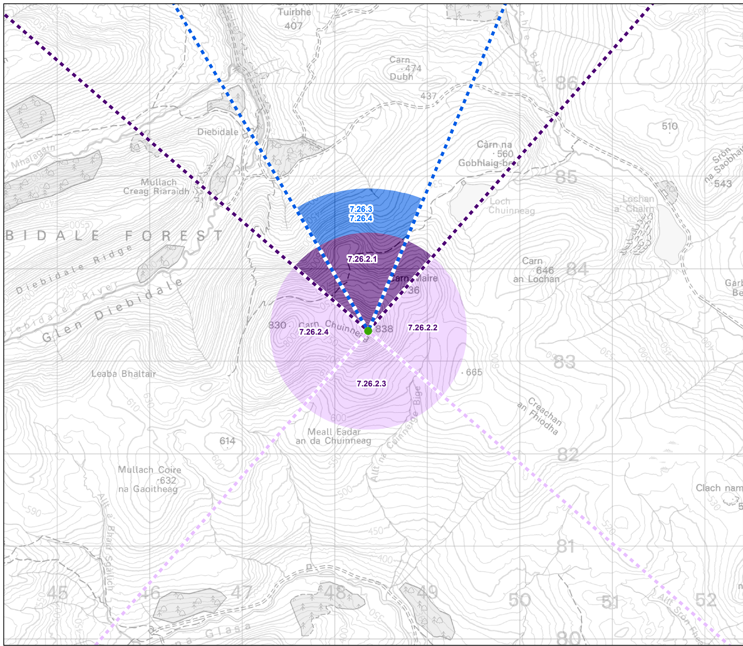
Figure 7.26.1 Viewpoint 18: Carn Chuinneag - Location Plan
