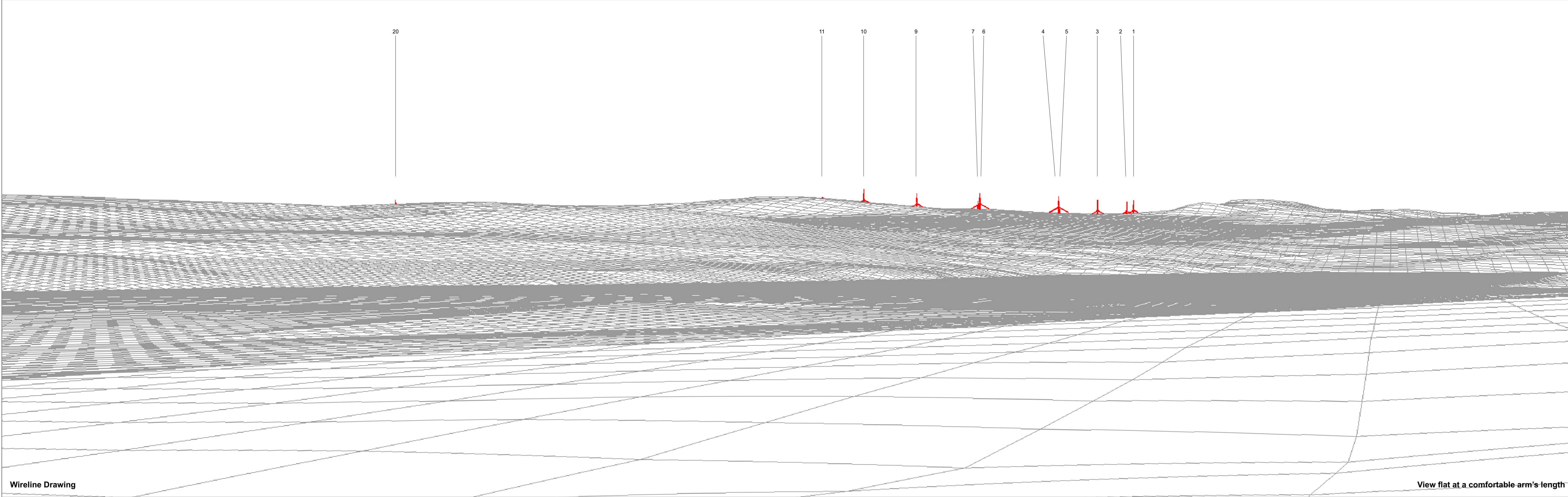
Achany Extension Wind Farm EIA Figure 7.17.3 - Viewpoint 9: Achnairn caravan and camping site entrance
