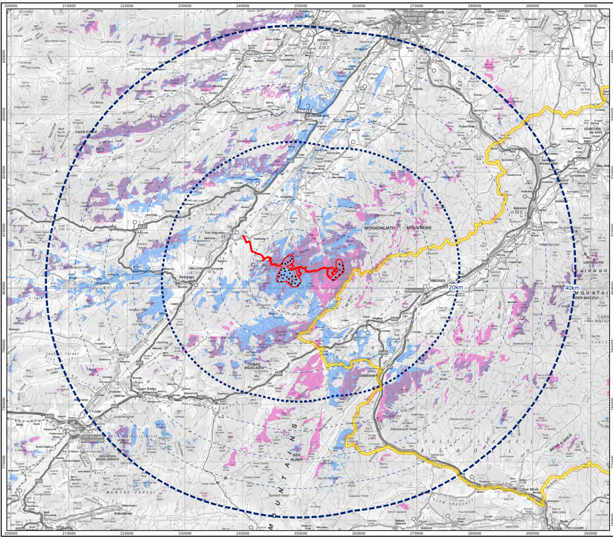
Figure 7.1.3 Comparative ZTV of Eastern and Western Clusters Cloiche Wind Farm EIA Report
