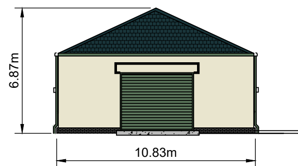
3. SIDE ELEVATION
