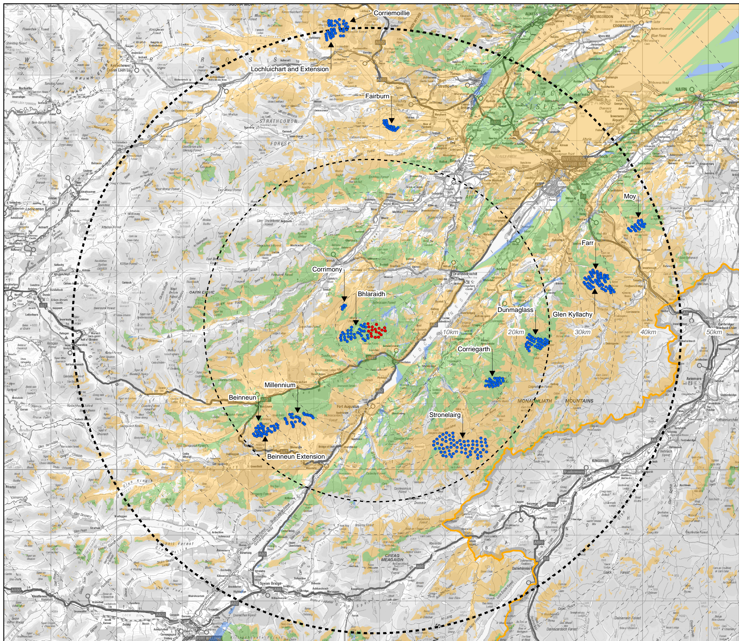
Figure 8.8.2 Cumulative ZTV - Proposed Development with Operational/Under Construction Sites
