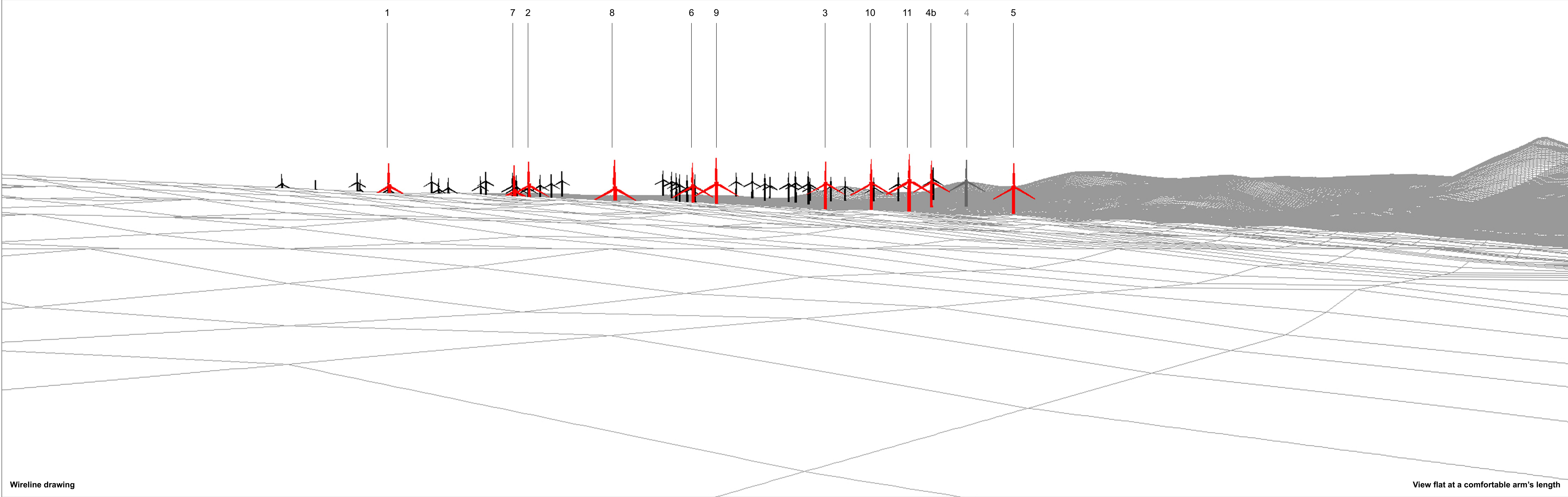
Gordonbush Extension Wind Farm Figure A11.2.4 - Comparative Wireline from Balnacoil Hill Cairn (53.5°)
