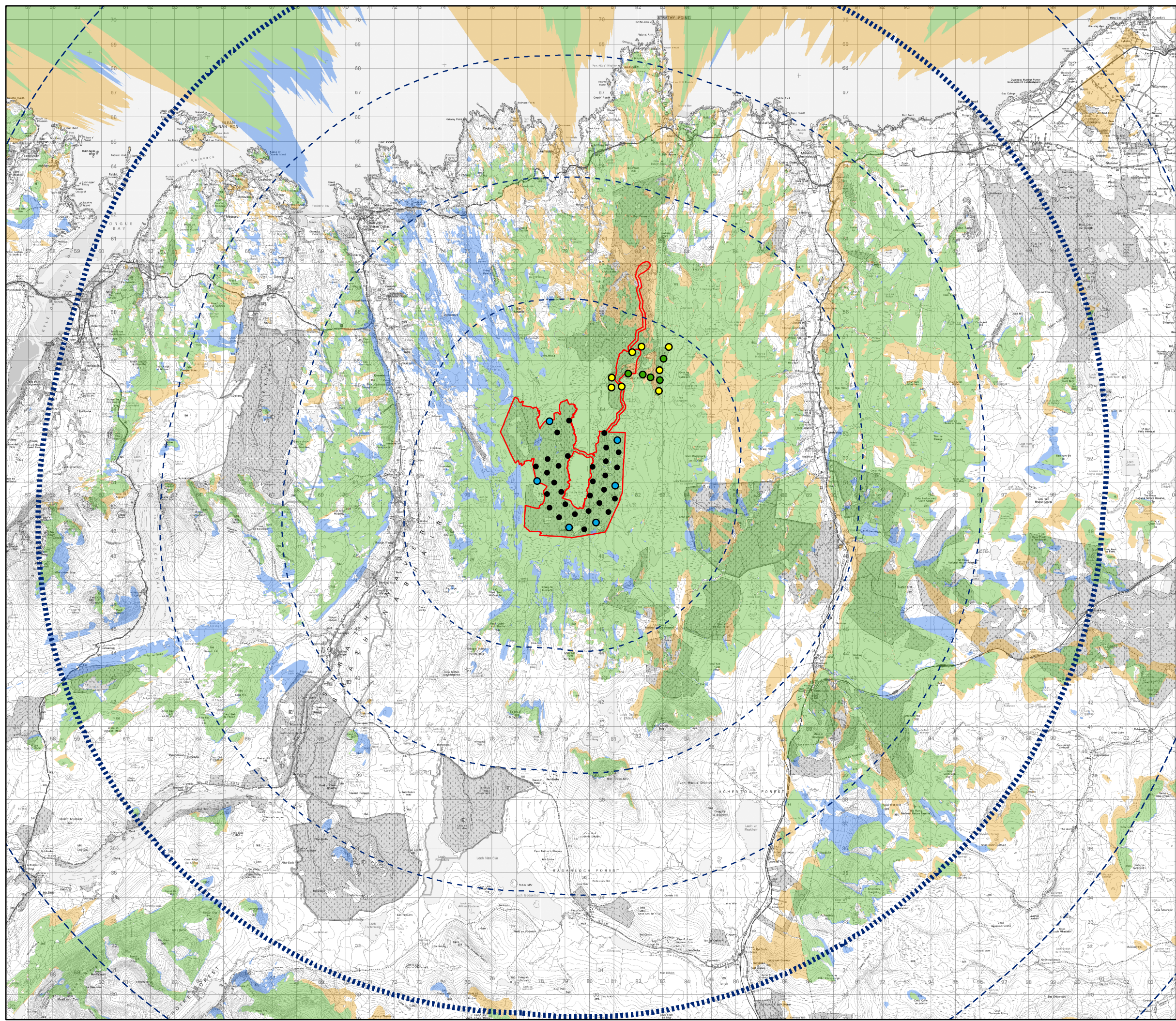
TA Figure 4.2.11 Cardinal Lighting Strategy: Comparative Hub Height ZTV (Strathy Wood)
