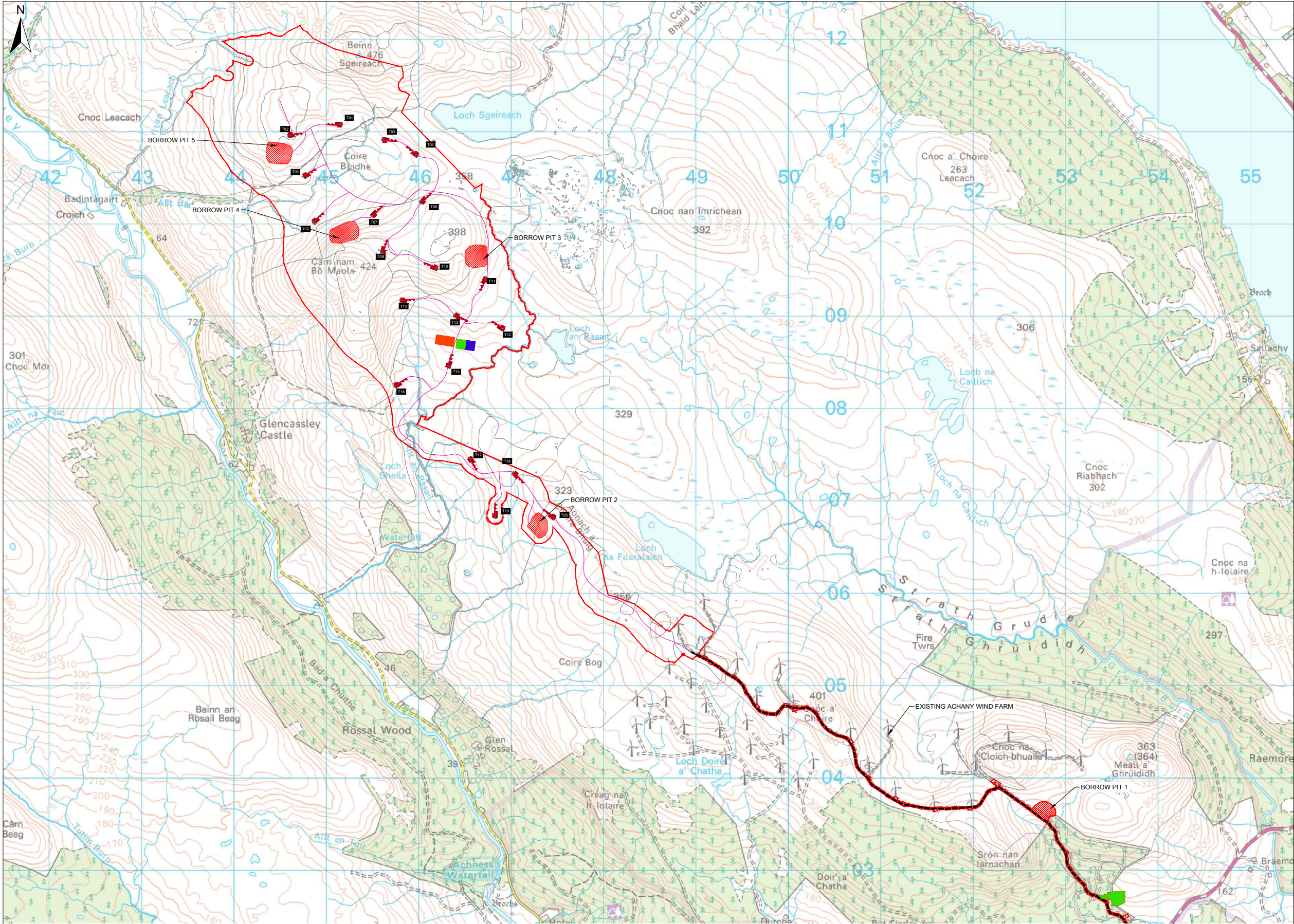
SITE LAYOUT SCALE 1:20000
