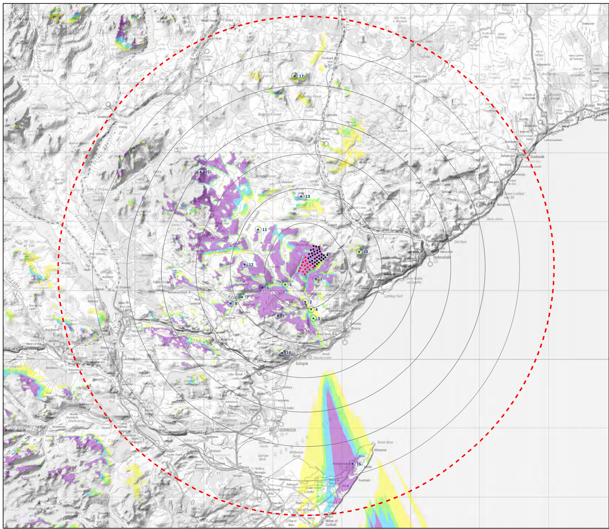
Figure 7.9a HUB HEIGHT ZTV WITH VIEWPOINTS
