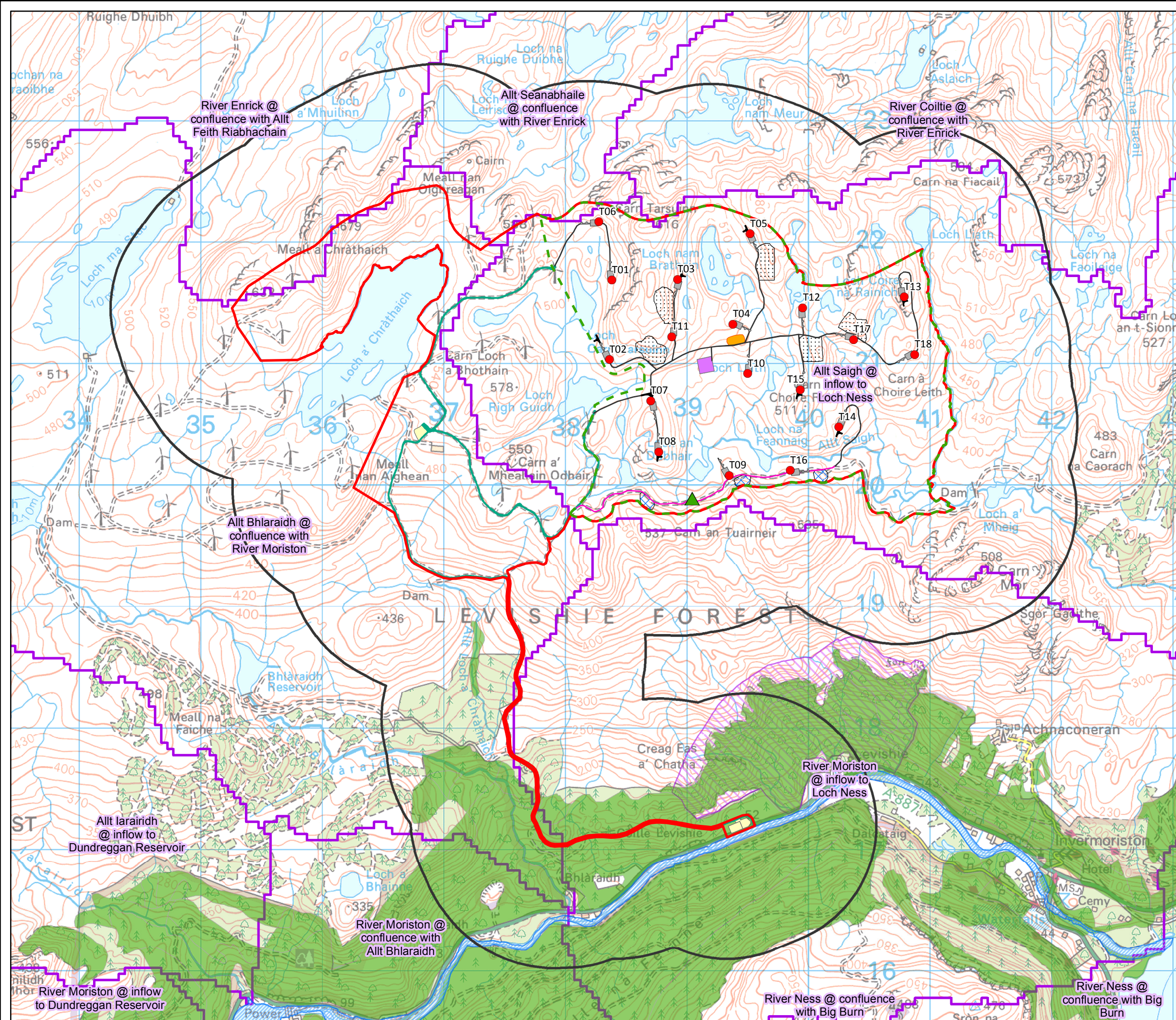
Figure 9.3 Environmental Constraints Bhlaraidh Wind Farm Extension EIA Report
