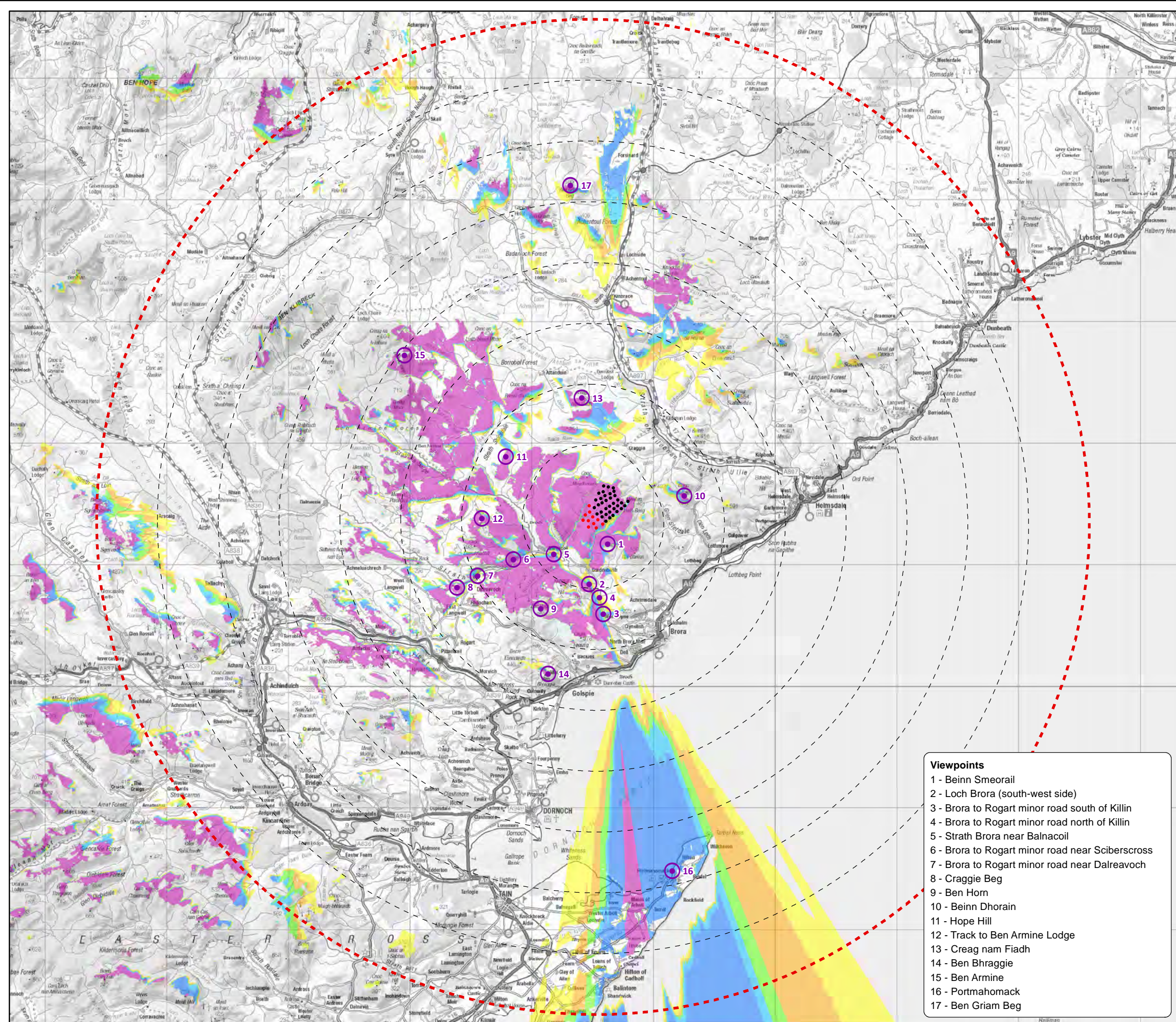
Figure 7.1a Blade Tip ZTV with Viewpoints Gordonbush Extension Wind Farm EIA Report
