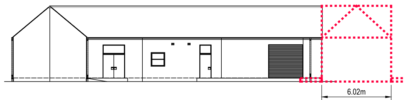
3. REAR ELEVATION
