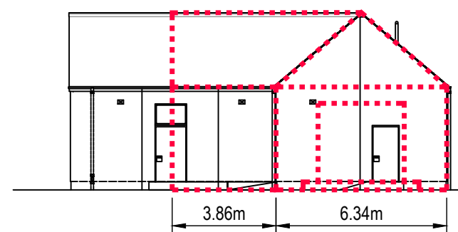
4. SIDE ELEVATION
