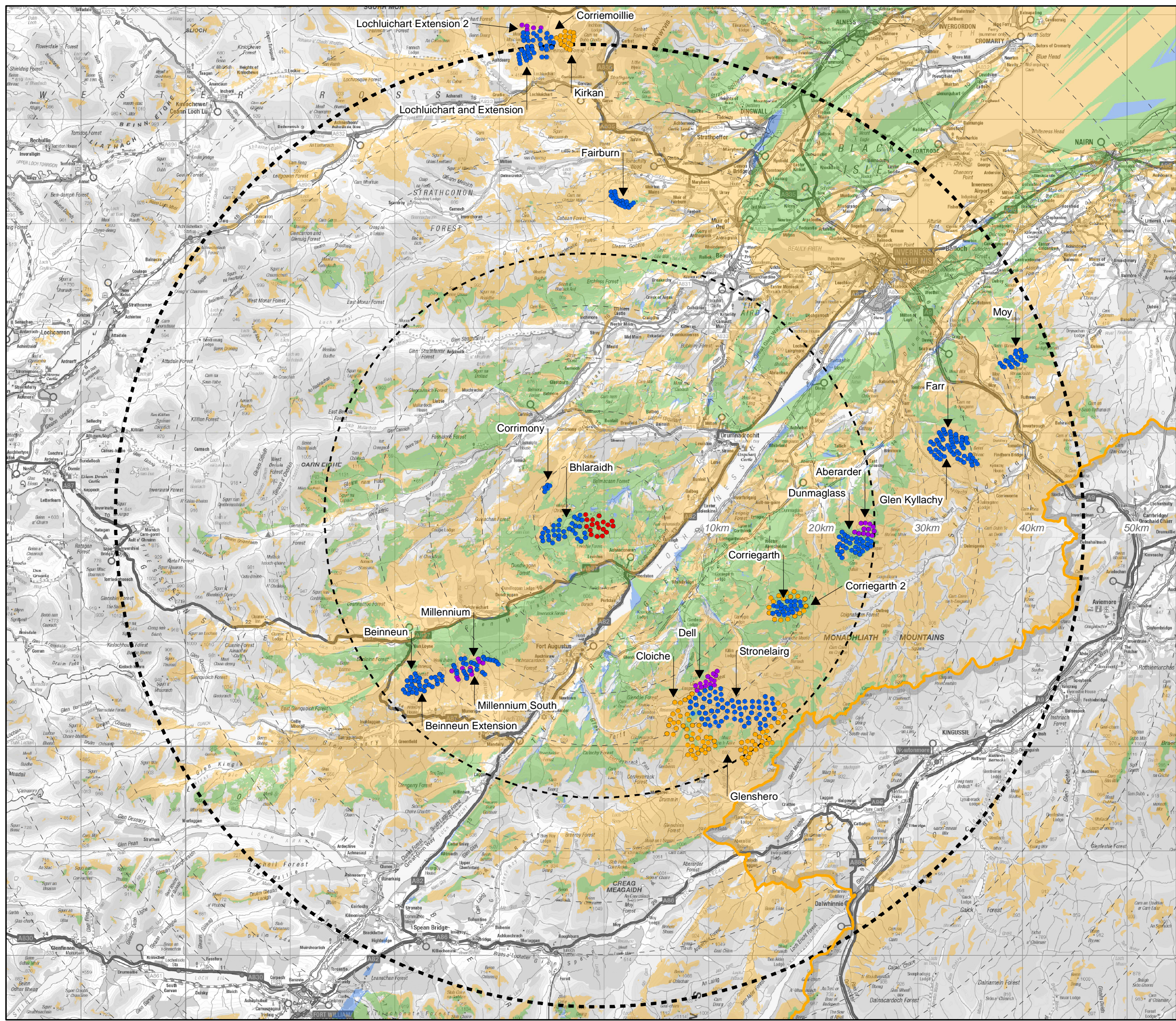
Figure 8.8.1 Cumulative ZTV - Proposed Development with All CLVIA Sites
