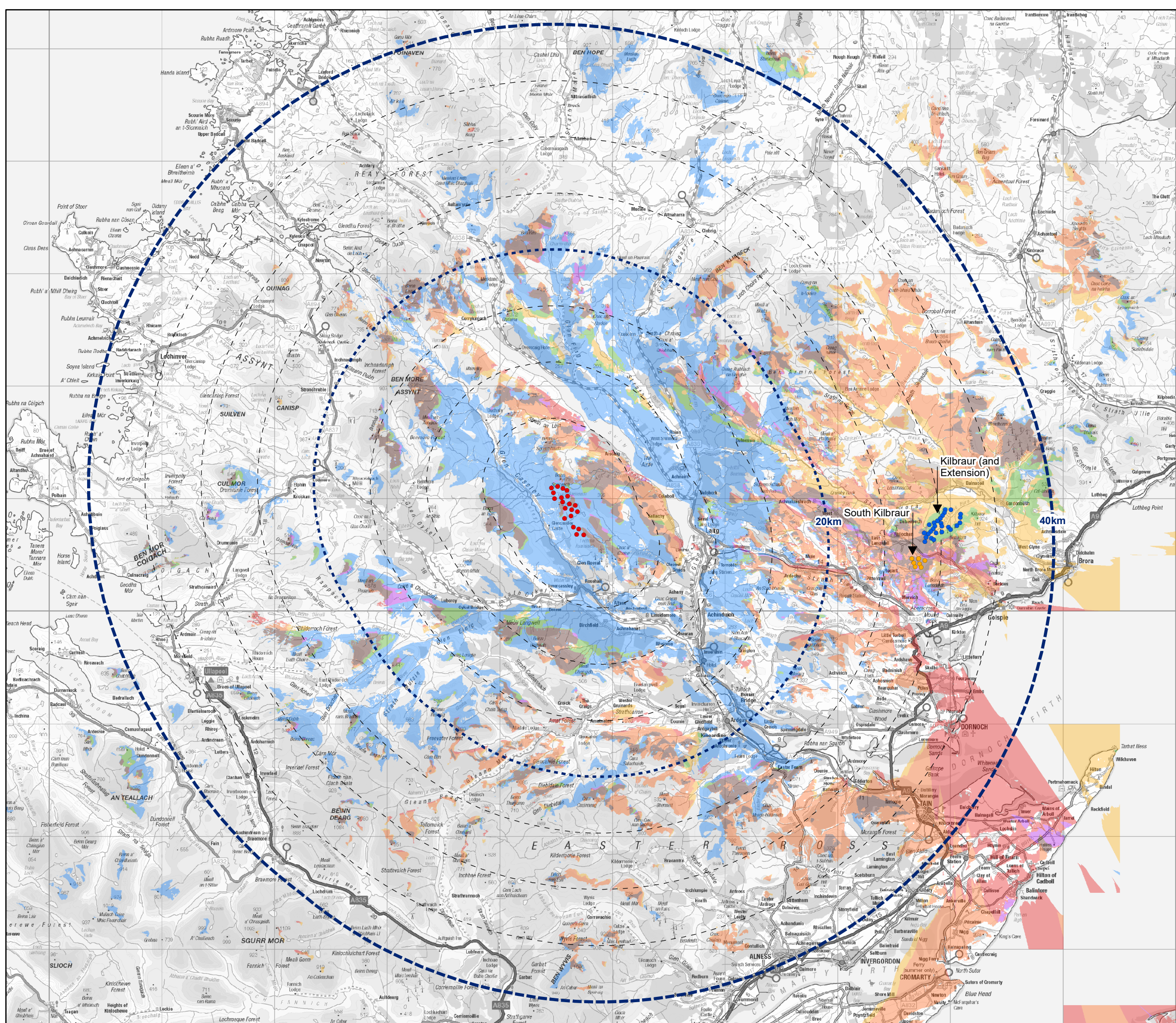
Figure 7.8.10 Cumulative ZTV - Proposed Development with Kilbraur (and Extension) and South Kilbraur
