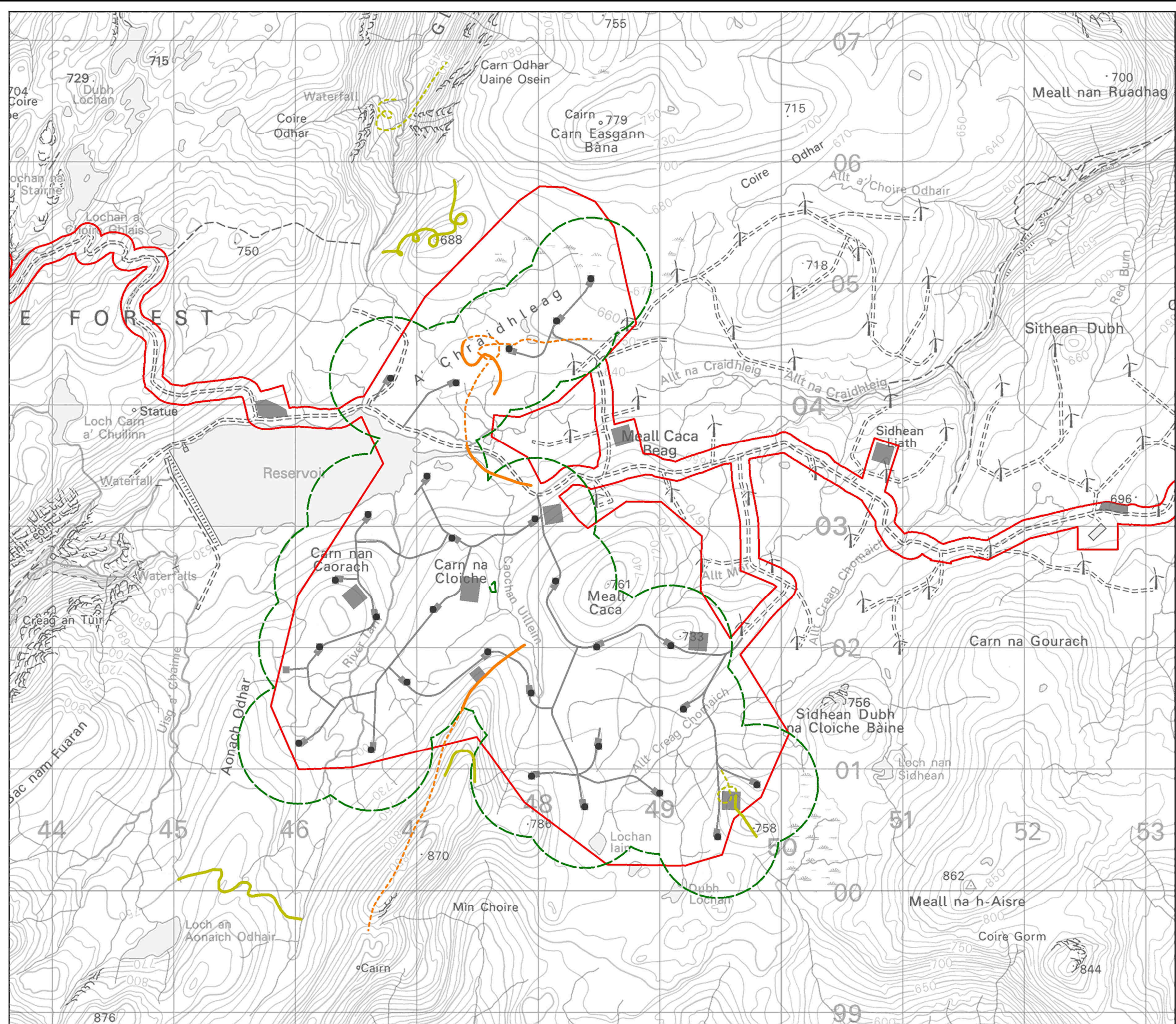
Figure 9.5a Flight Activity by Golden Eagle (Aug 2018-Jan 2019, Western Cluster)
