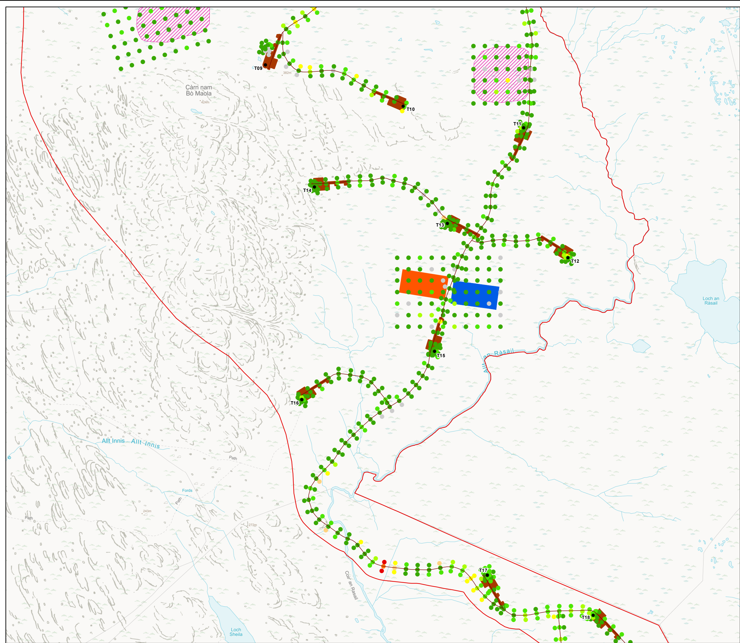
Figure 11.3D Peat Depth Achany Extension Wind Farm EIA Report
