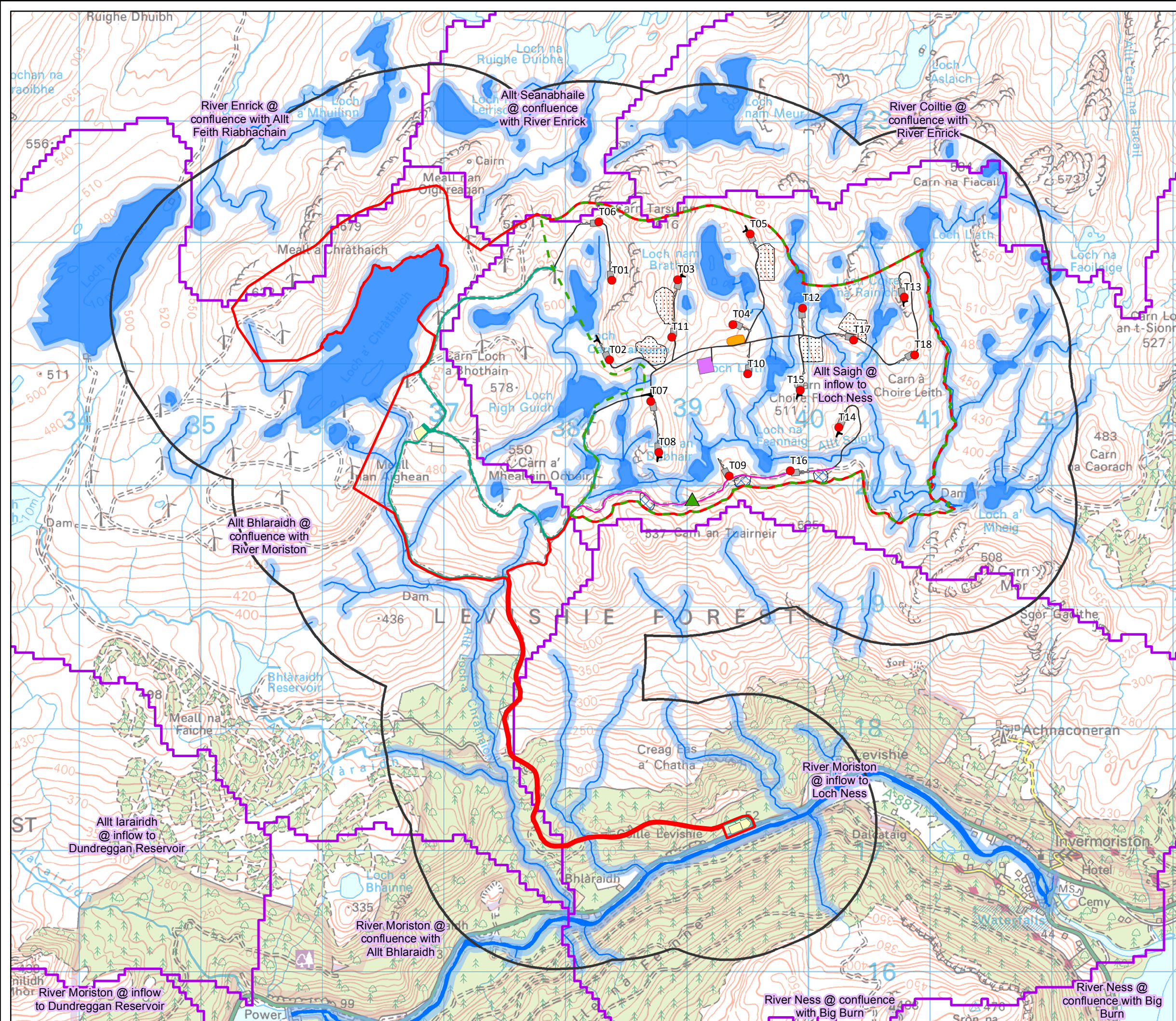
Figure 9.2 Hydrological Overview Bhlaraidh Wind Farm Extension EIA Report
