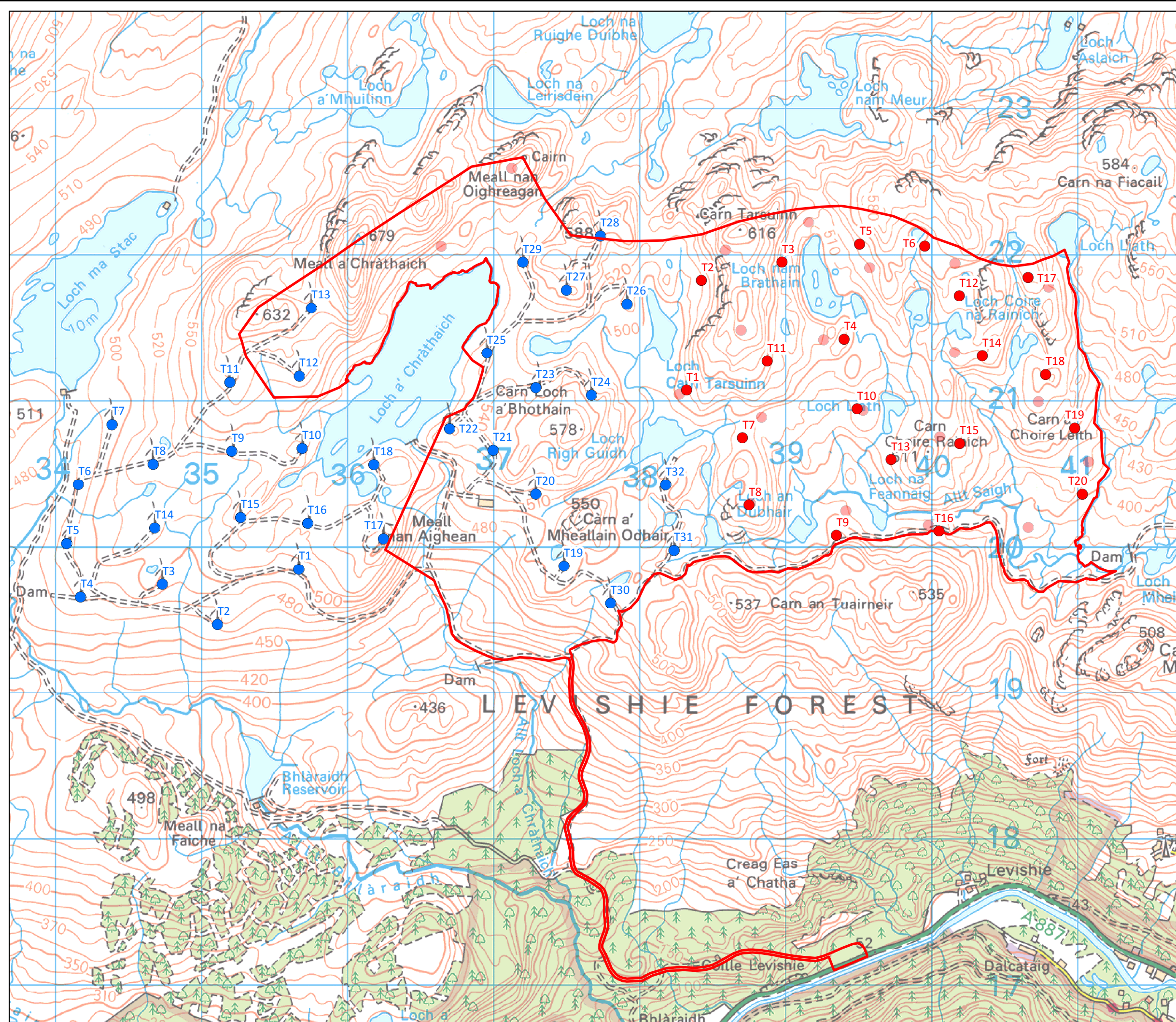
Figure 2.2 Layout B Bhlaraidh Wind Farm Extension EIA Report
