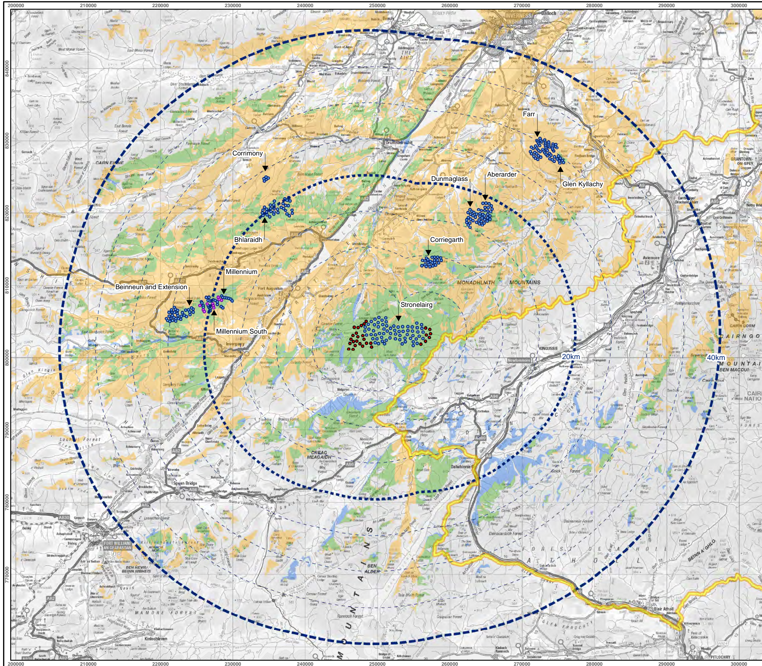
Figure 3.7.3 Cumulative ZTV - 29 Turbine Proposed Development with Operational/Under Construction and Consented Sites Cloiche Wind Farm Additional Information
