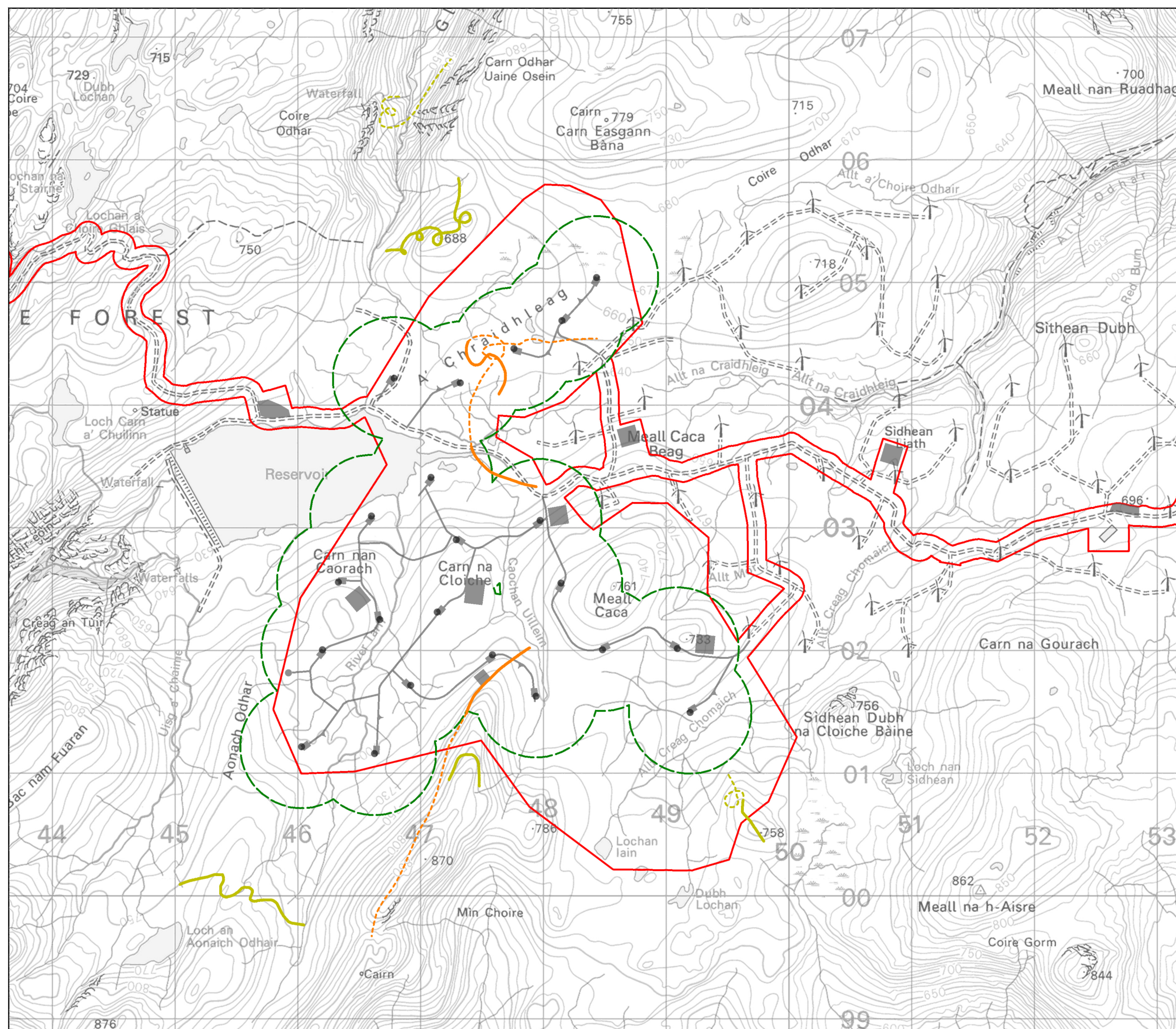
Figure 5.5a Flight Activity by Golden Eagle (Aug 2018-Jan 2019, Western Cluster)
