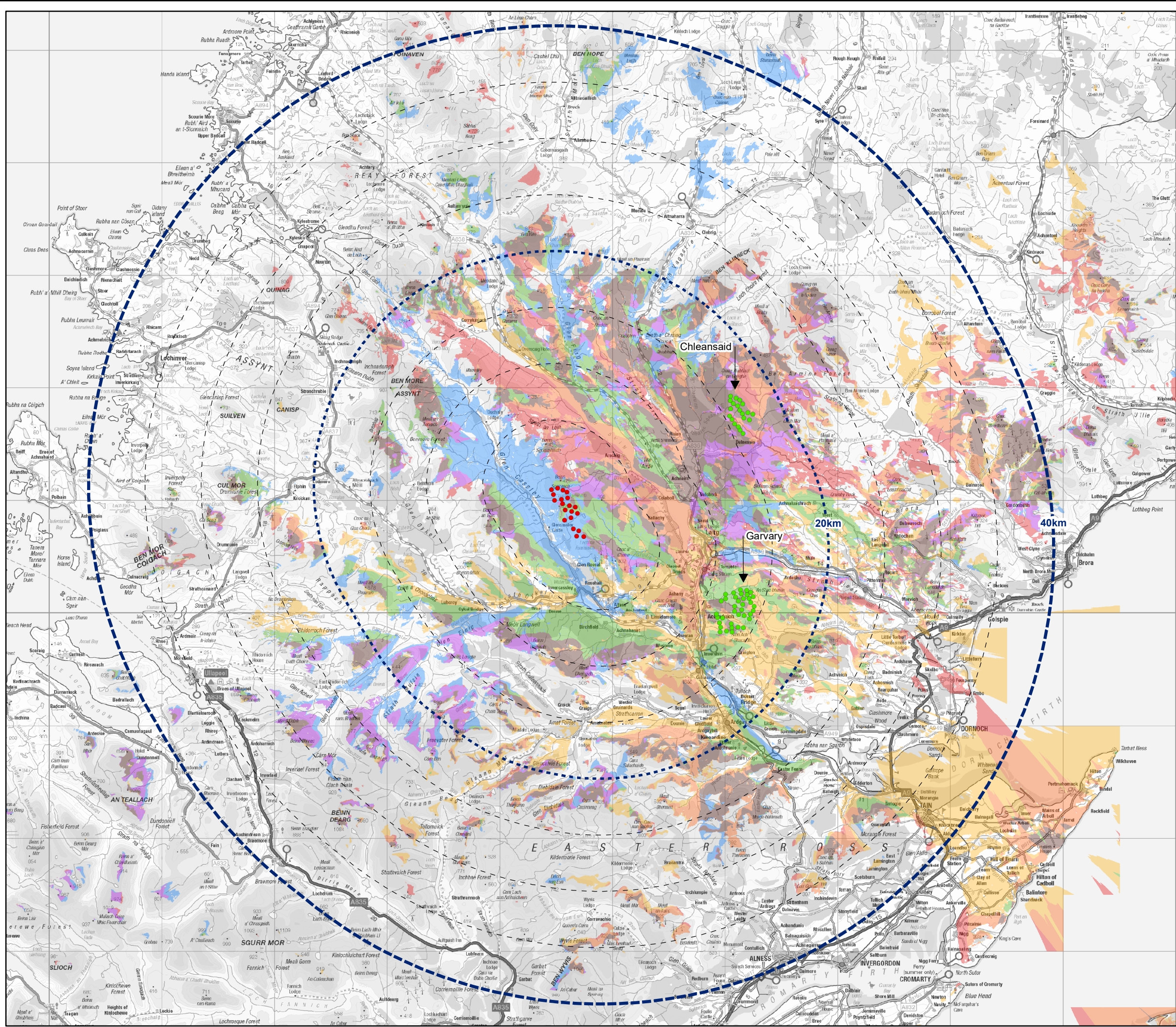
Figure 7.8.17 Cumulative ZTV - Proposed Development with Garvary and Chleaisaid
