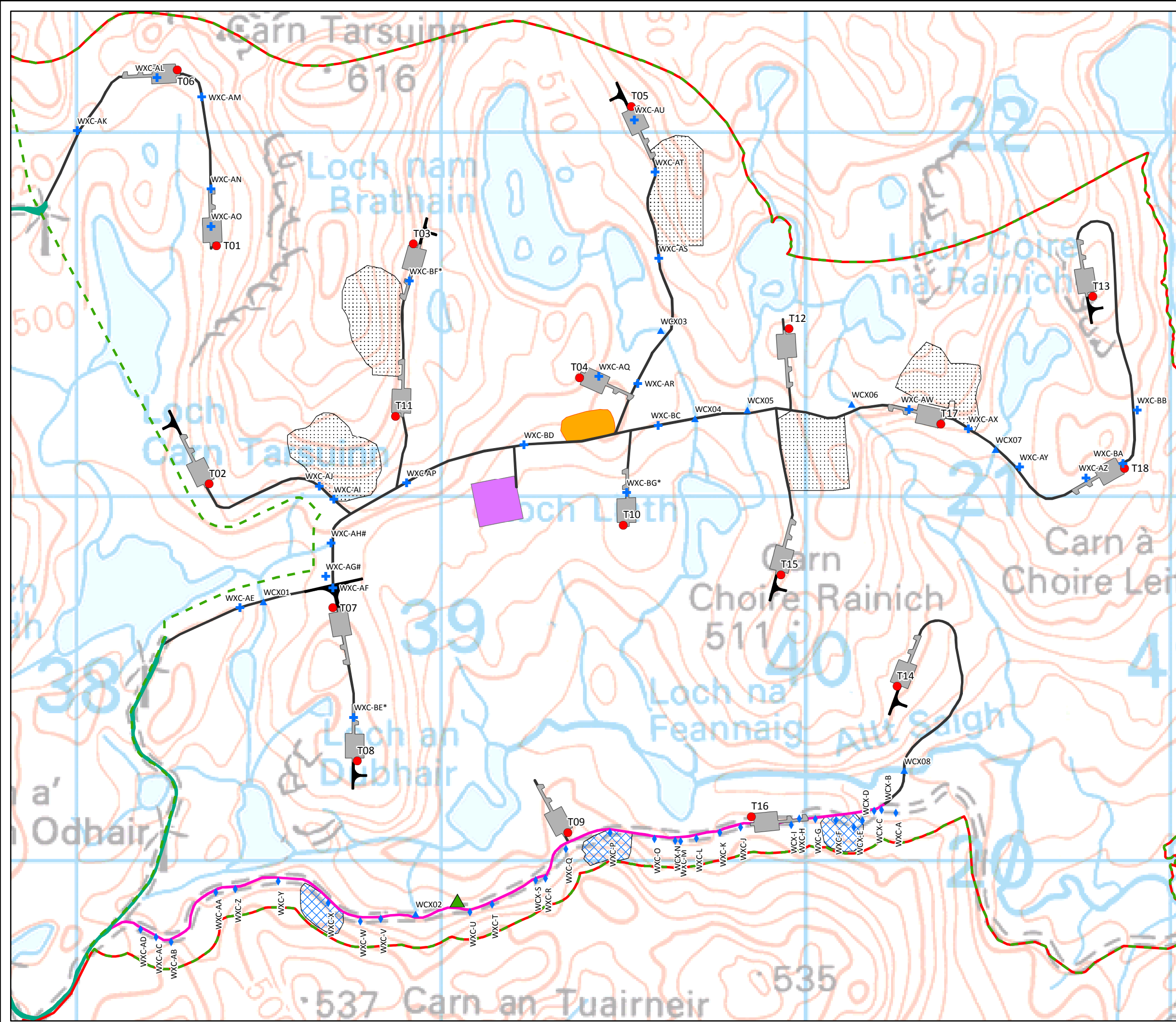
Figure 9.4 Watercourse Crossings Bhlaraidh Wind Farm Extension EIA Report
