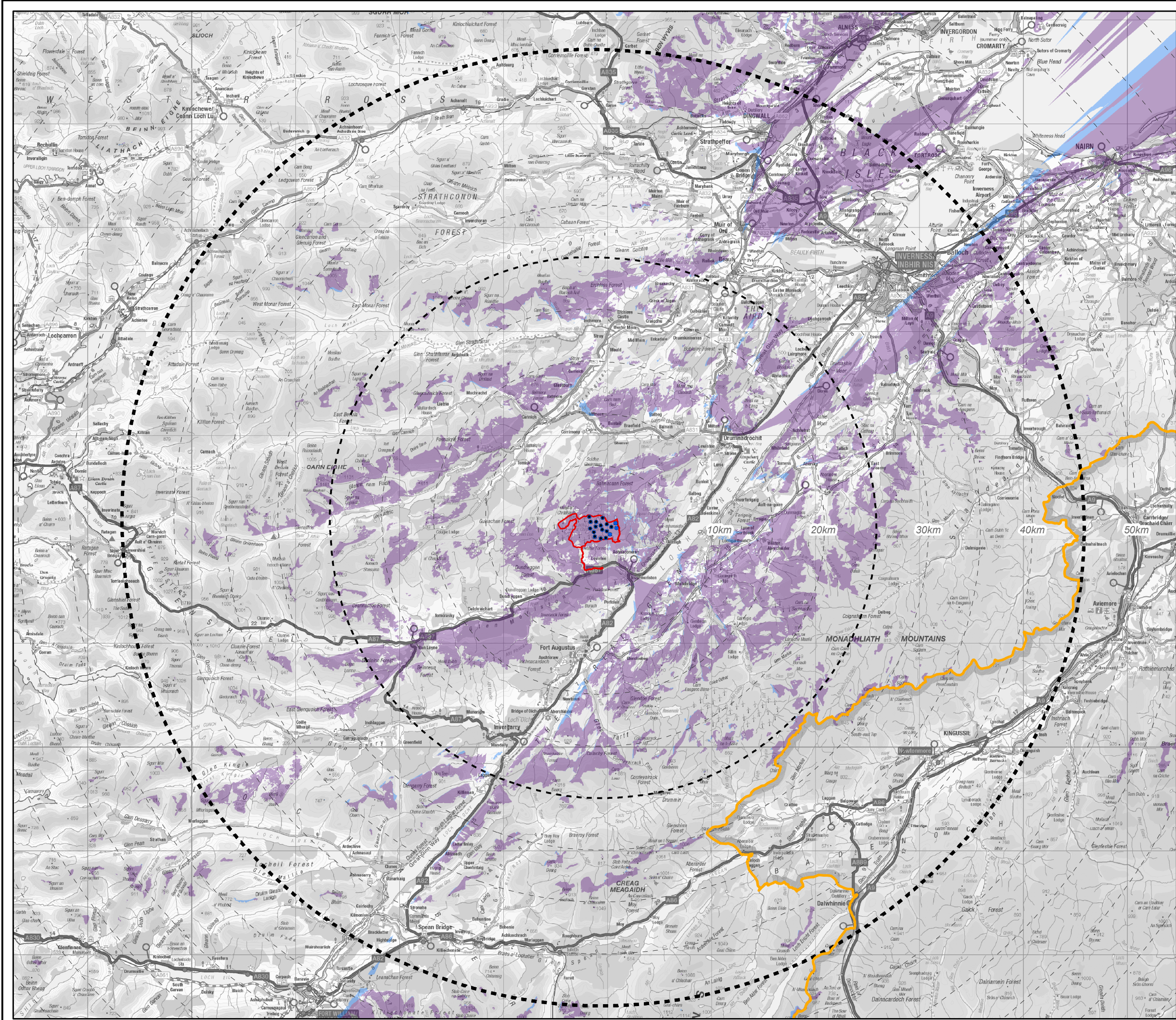
Figure 8.1.2 Comparative ZTV – 15 Turbine Layout with 18 Turbine Layout Bhlaraidh Wind Farm Extension Additional Information Report
