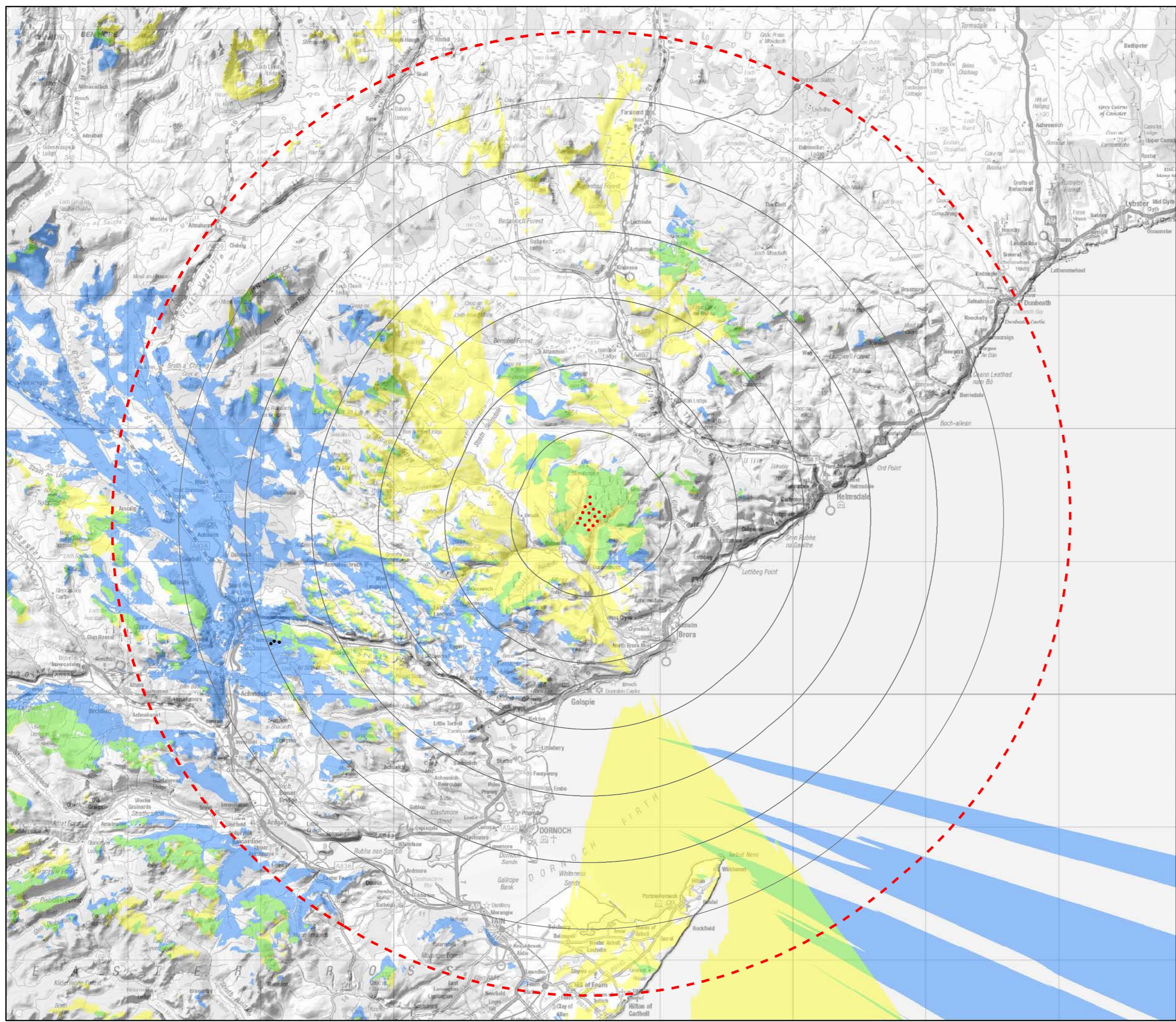
Figure 7.16f CUMULATIVE ZTV WITH LAIRG Gordonbush Extension Wind Farm Environmental Statement
