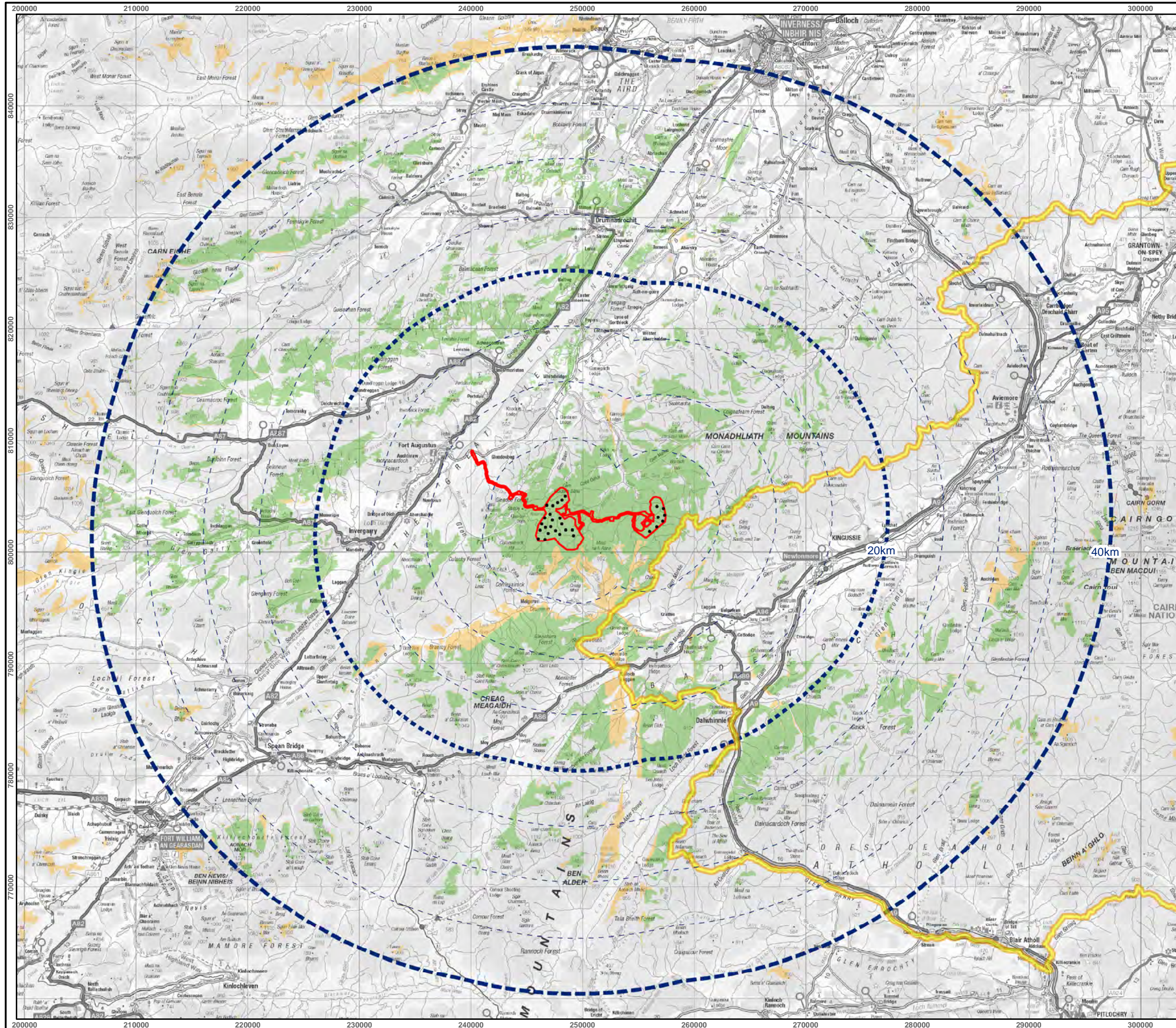
Figure 3.2 29 Turbine Proposed Development and the 36 Turbine Scheme Comparative ZTV
