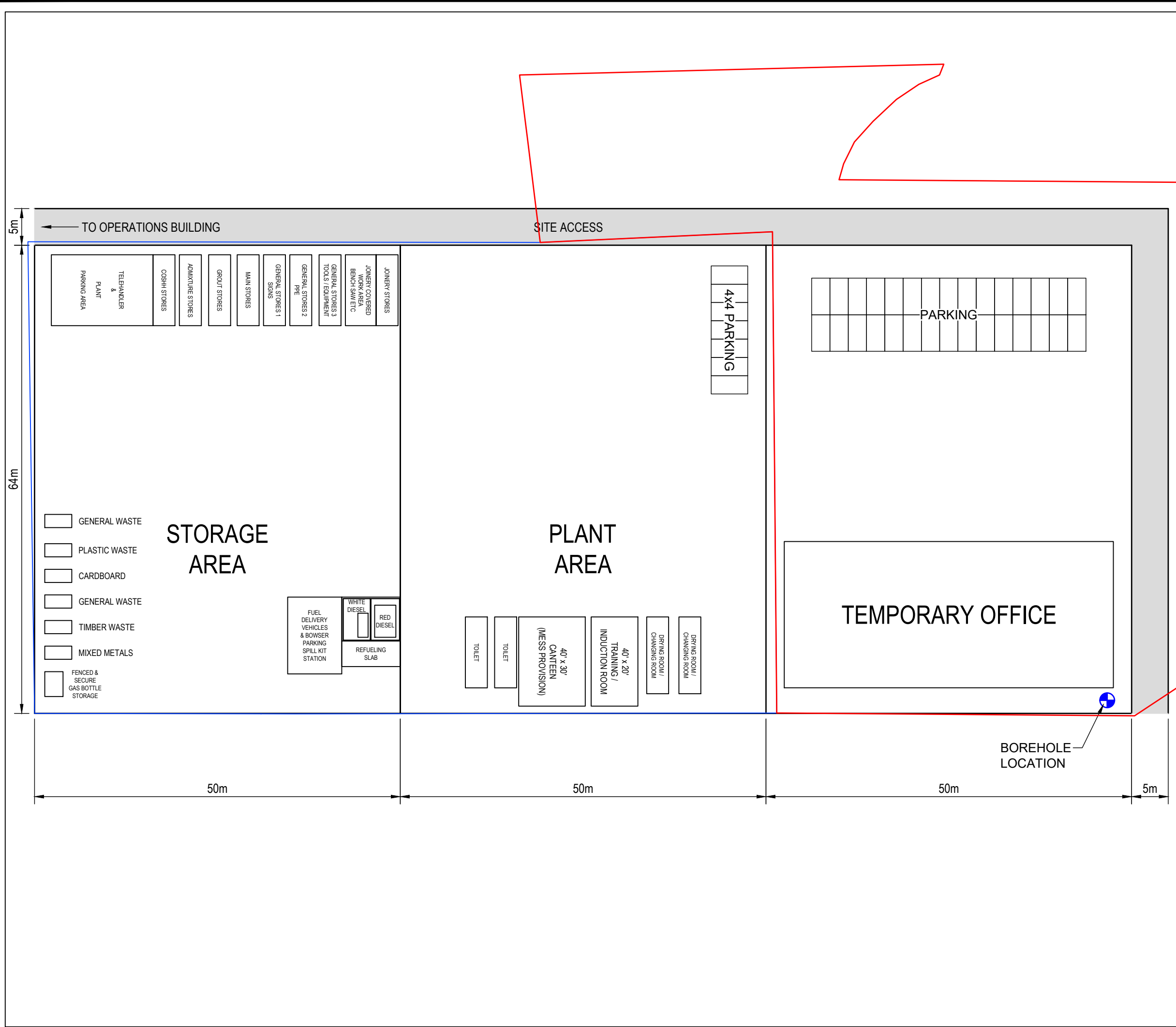
Figure 2.14 Typical Construction Compound Bhlaraidh Wind Farm Extension EIA Report
