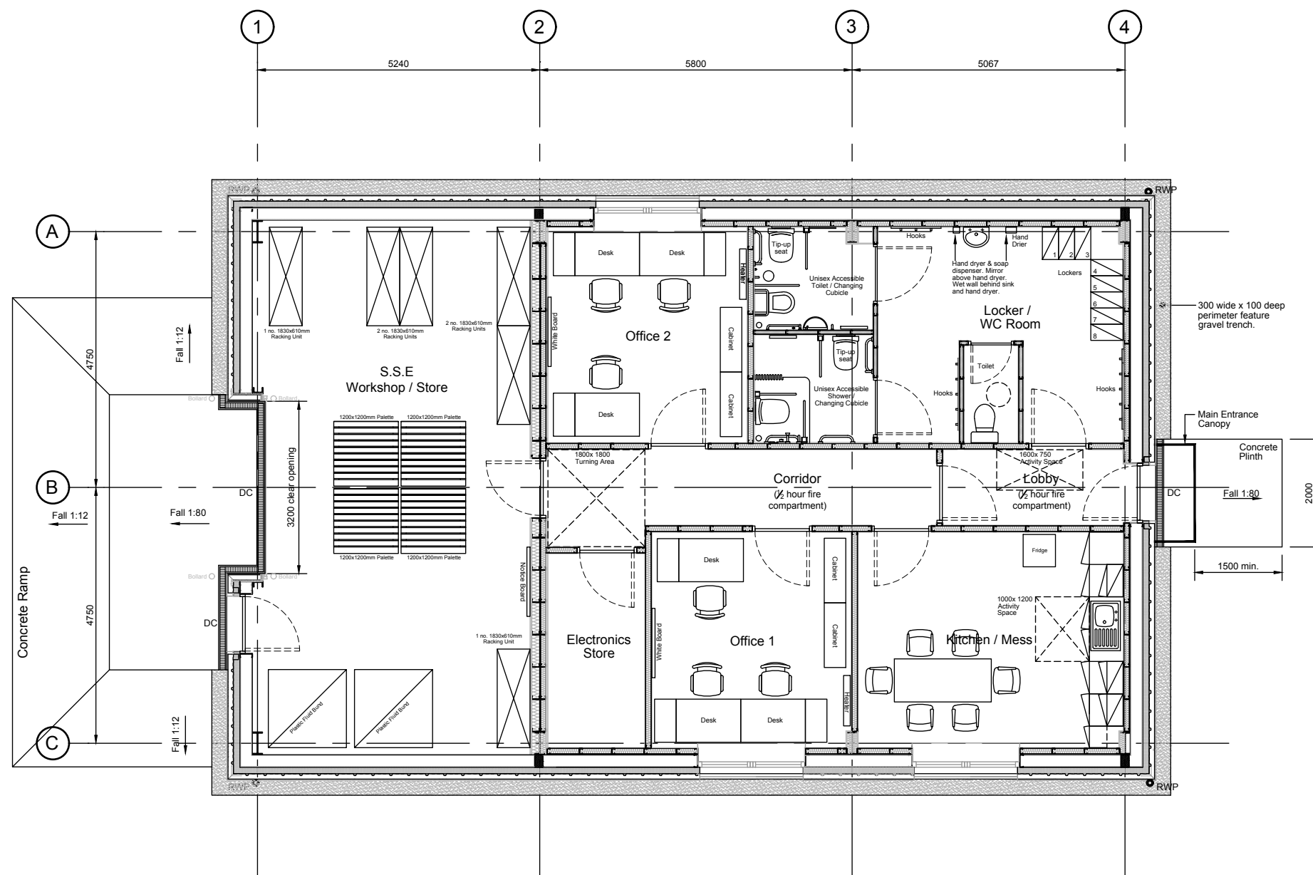
OL 01 : 6 to 20 Turbine Sites Scale 1:100
