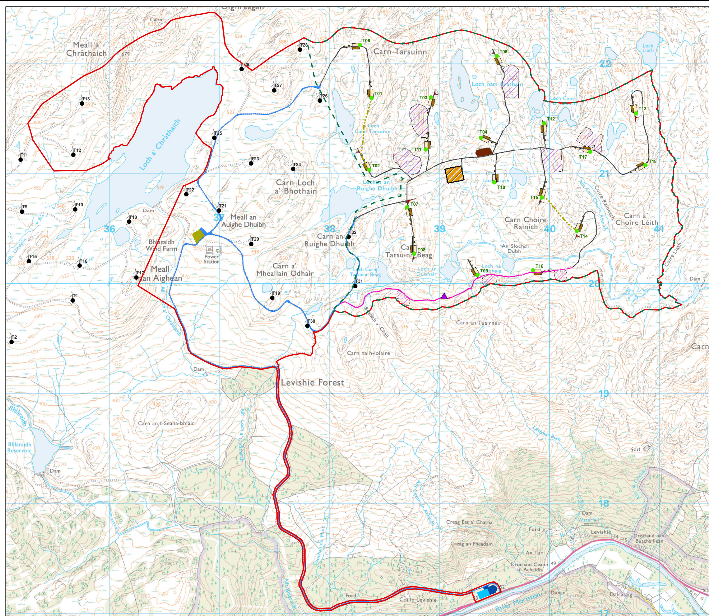
Figure 1.3 Site Layout Plan Bhlaraidh Wind Farm Extension EIA Report
