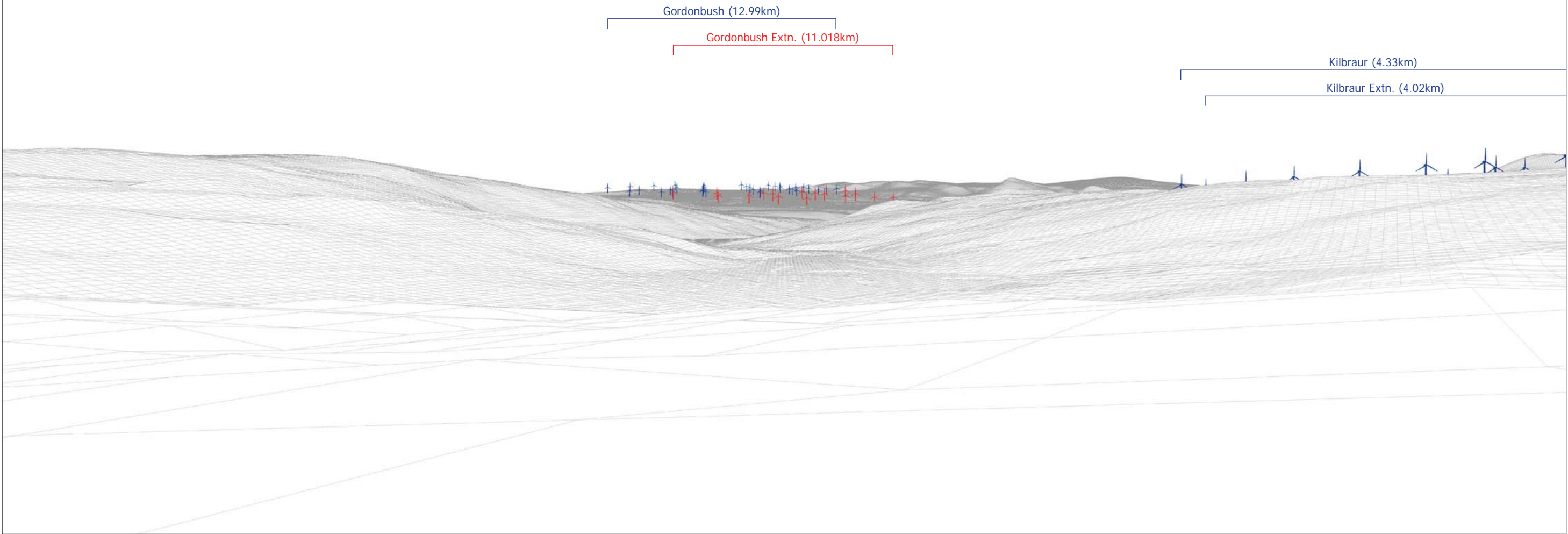
Viewpoint 8 Cumulative Wireline. Application turbines in red and operational / under construction in blue.
