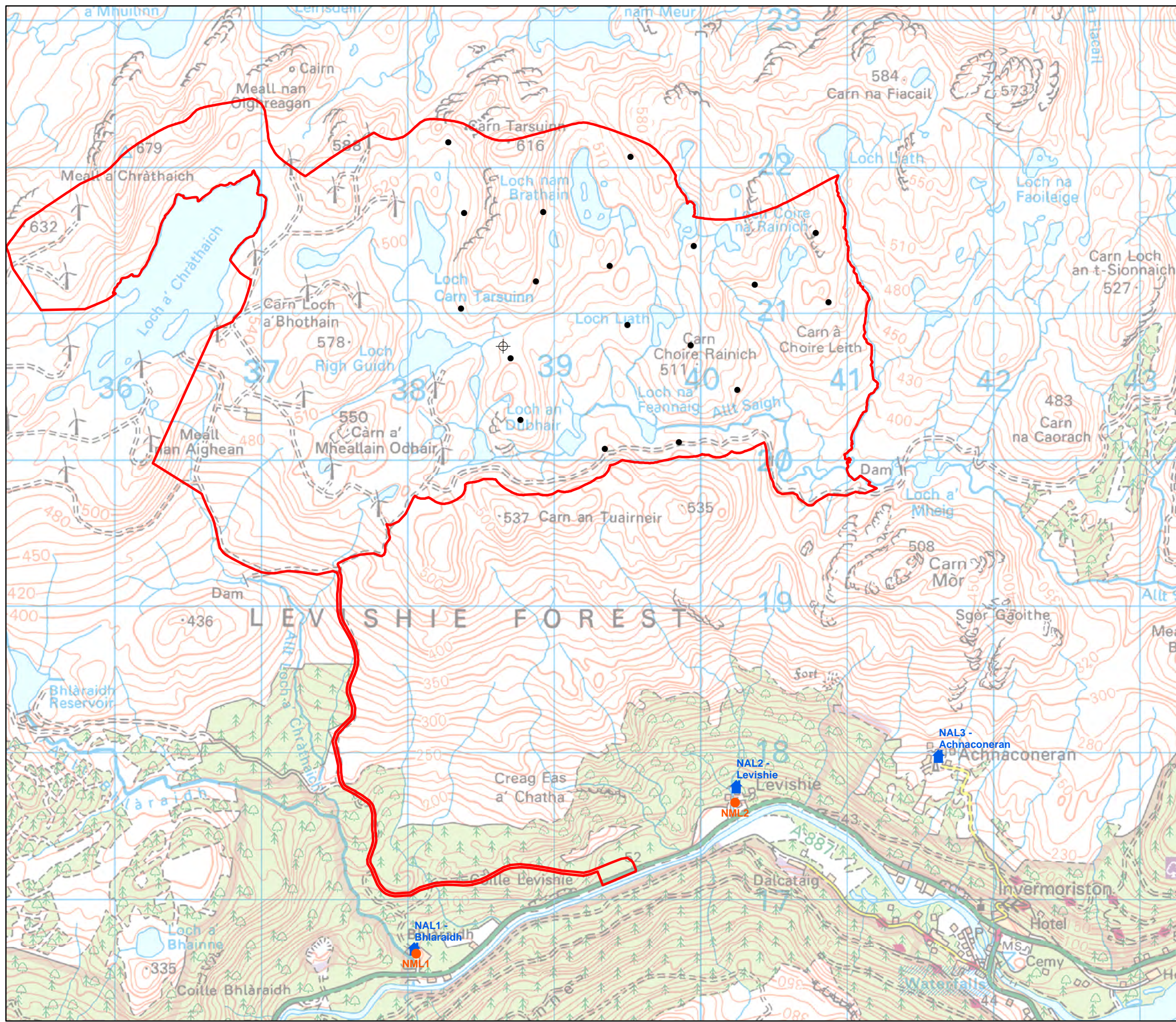
Figure 11.1 Noise Monitoring and Assessment Locations Bhlairaidh Wind Farm Extension EIA Report
