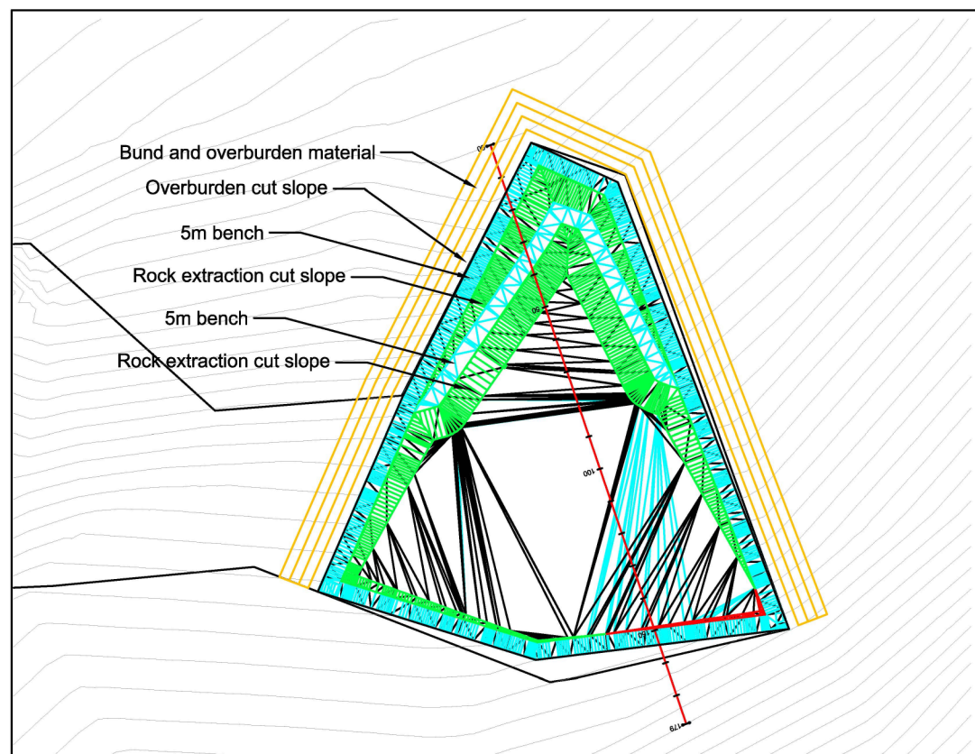
Borrow Pit A Plan Scale 1:2000
