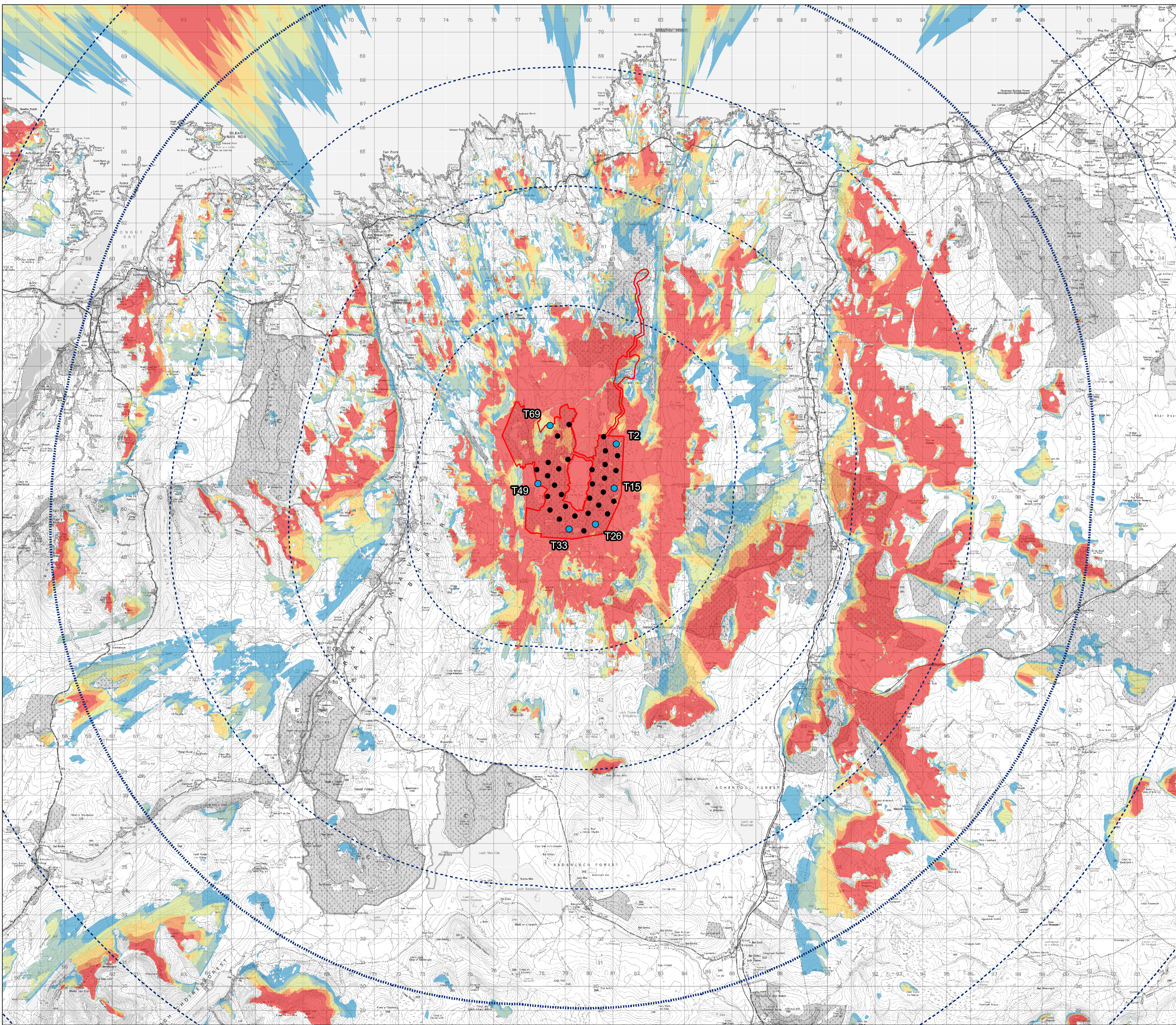
TA Figure 4.2.1b Cardinal Aviation Lighting Strategy: Hub Height ZTV (A1)
