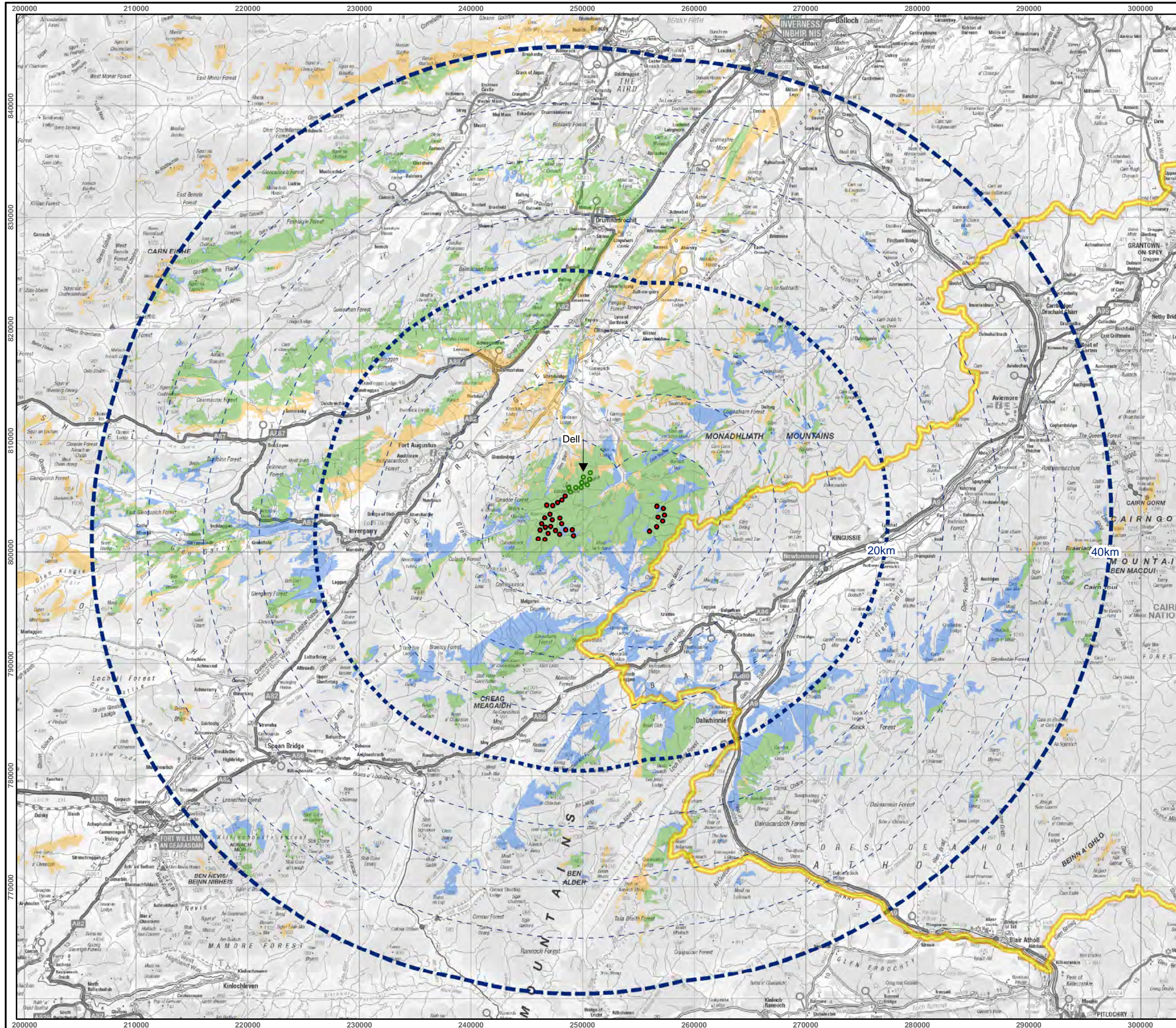
Figure 3.7.4 29 Turbine Proposed Development with Dell Cloiche Wind Farm Additional Information
