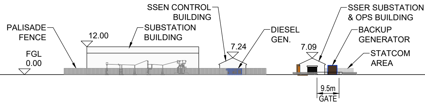
2. RIGHT ELEVATION
