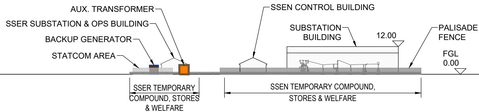
4. LEFT ELEVATION
