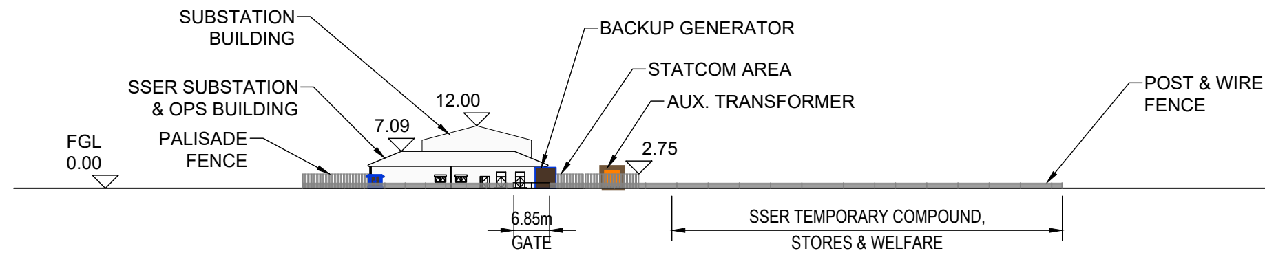
1. FRONT ELEVATION
