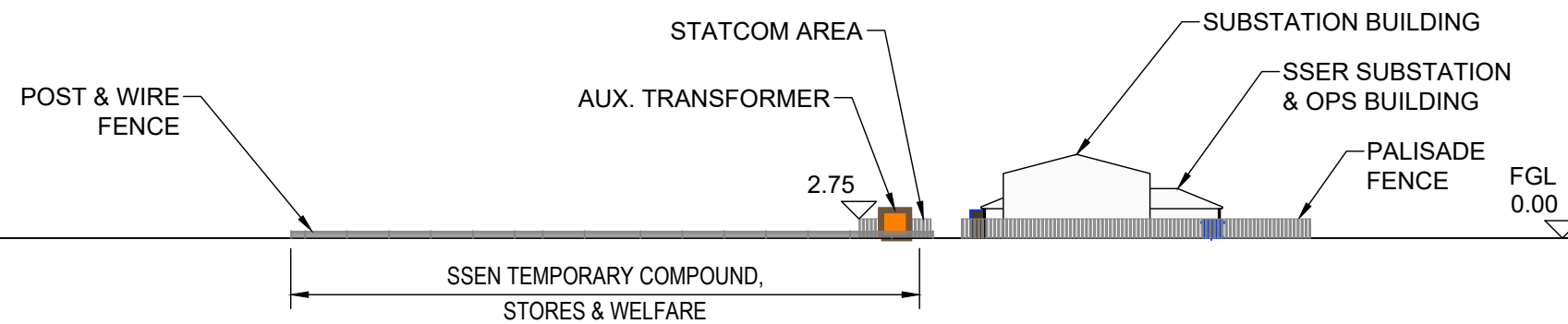
3. BACK ELEVATION
