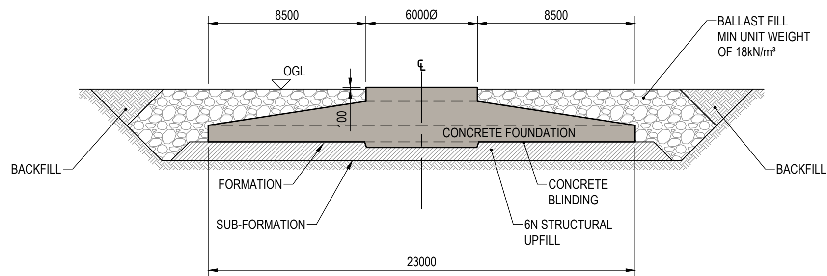
SECTION THROUGH INDICATIVE TURBINE FOUNDATION
