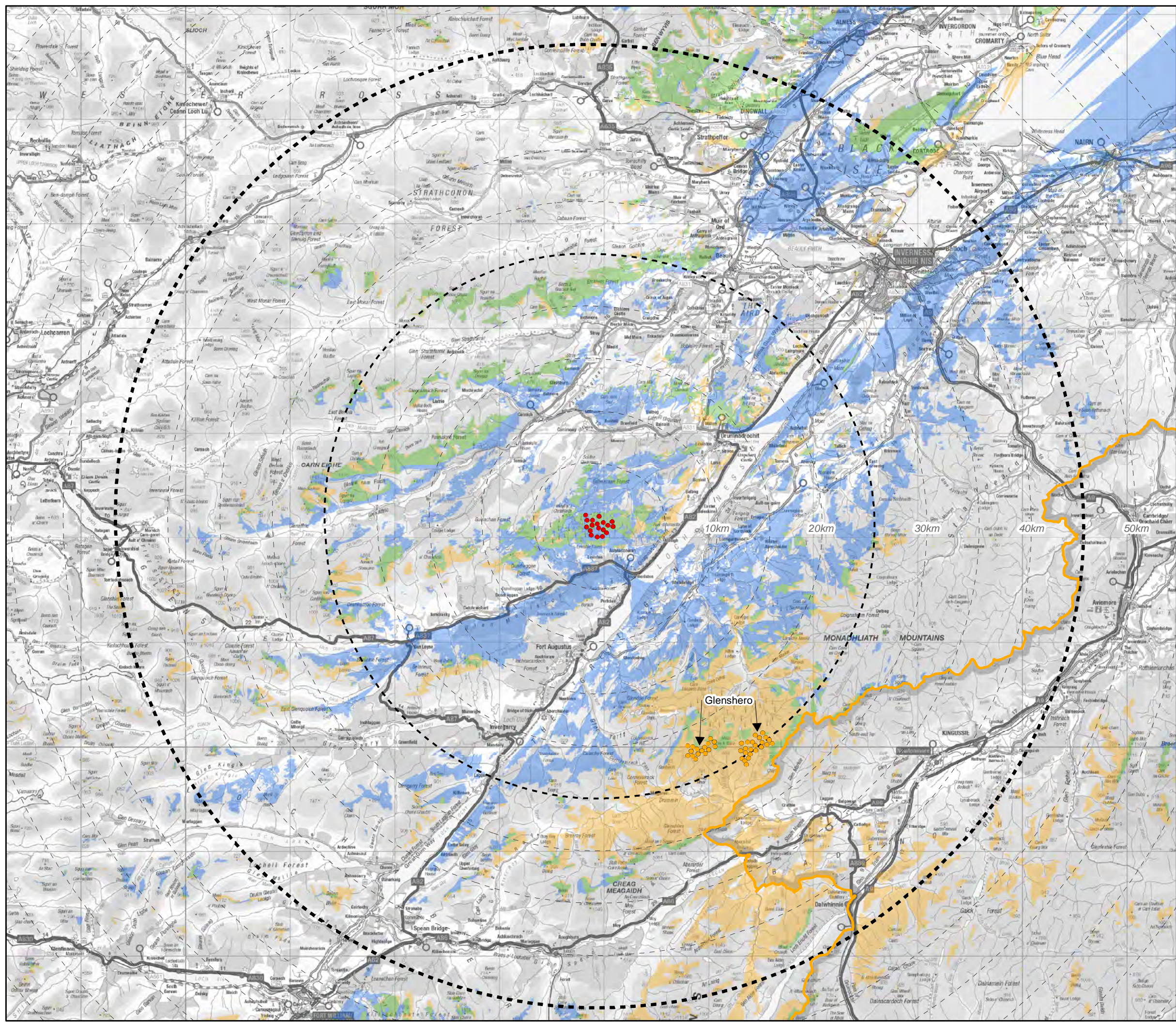
Figure 8.8.23 Cumulative ZTV - Proposed Development with Glenshero Bhlaraidh Wind Farm Extension EIA Report
