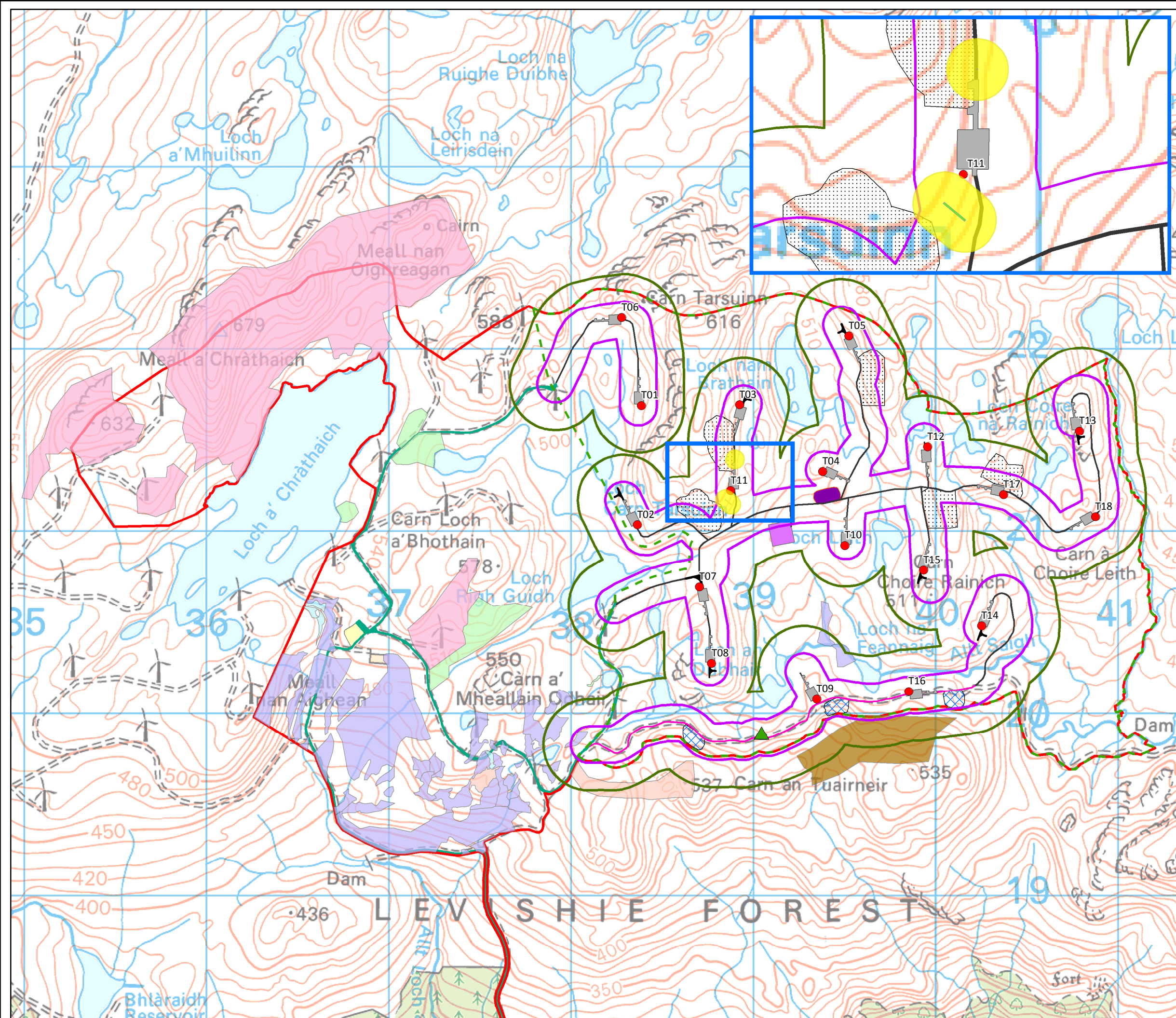
Figure 9.6 Assessed Groundwater Dependent Terrestrial Ecosystems Bhlaraidh Wind Farm Extension EIA Report
