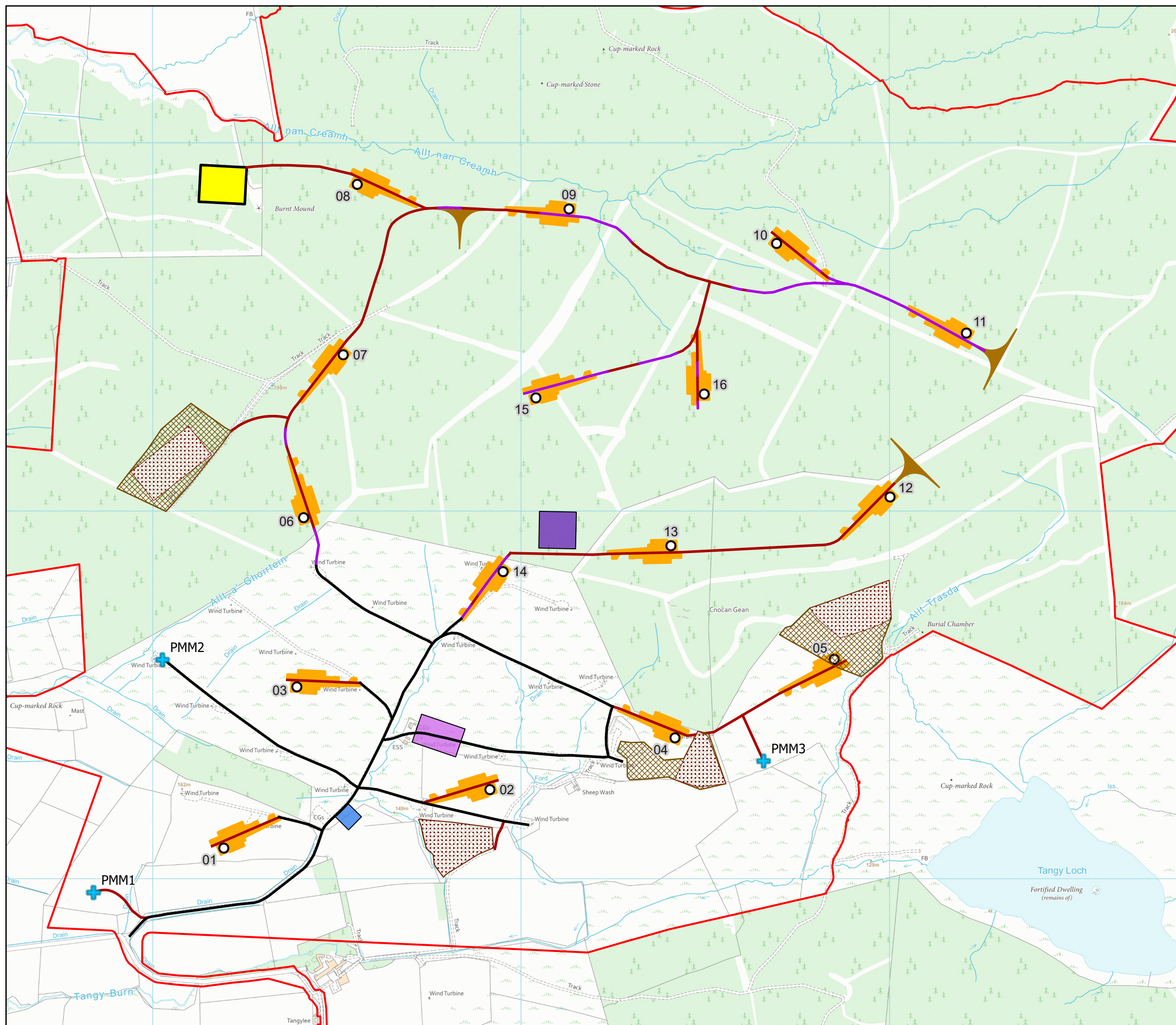
Figure 1 Proposed Varied Development Layout
