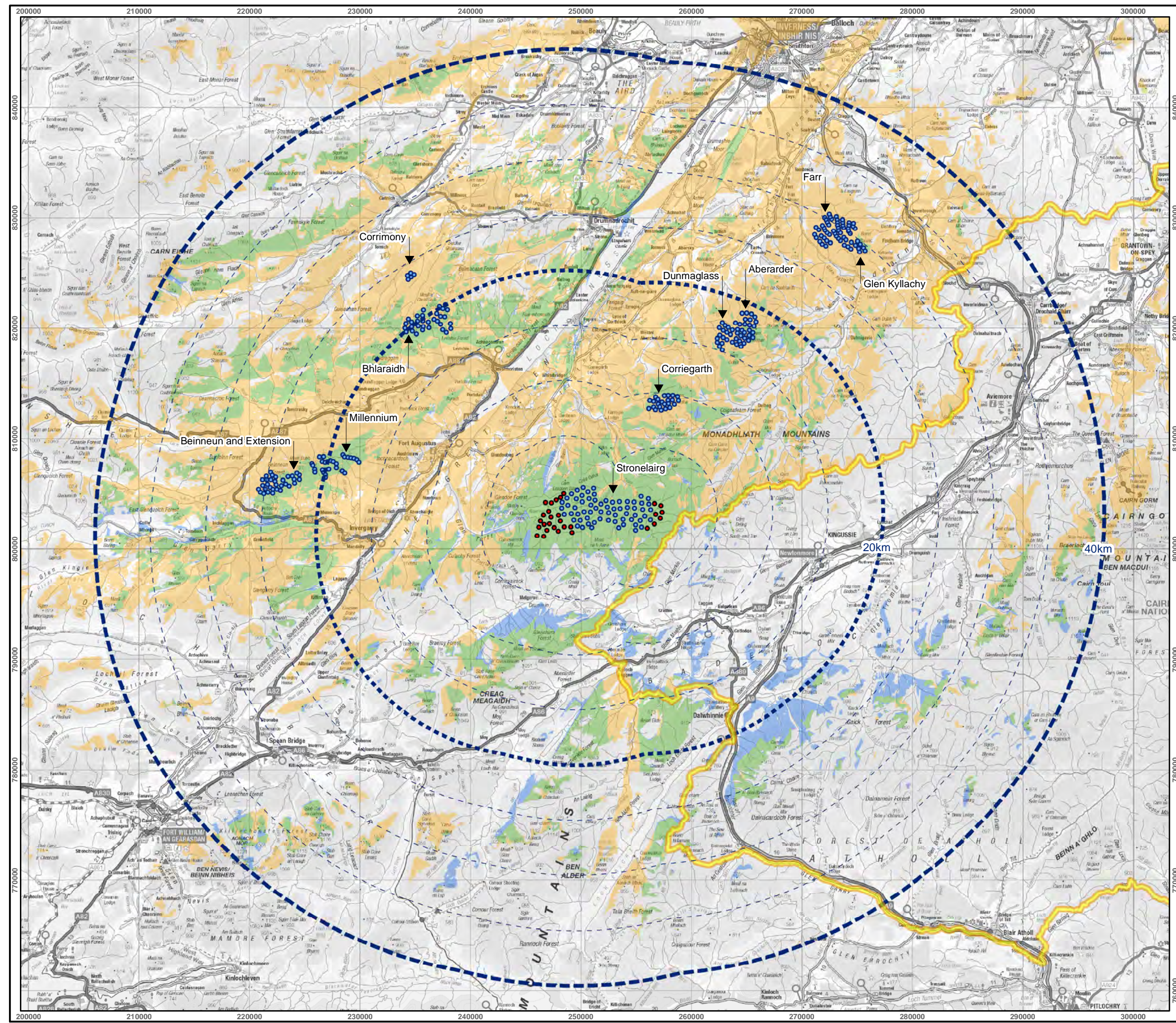
Figure 3.7.2 Cumulative ZTV - 29 Turbine Proposed Development with Operational/Under Construction Sites
