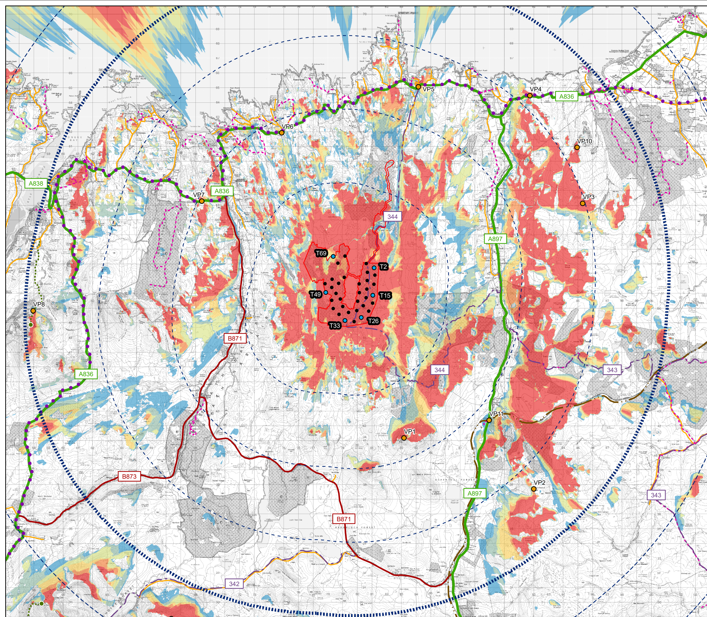
TA Figure 4.2.4 Cardinal Aviation Lighting Strategy: Visual Receptors with Hub Height ZTV
