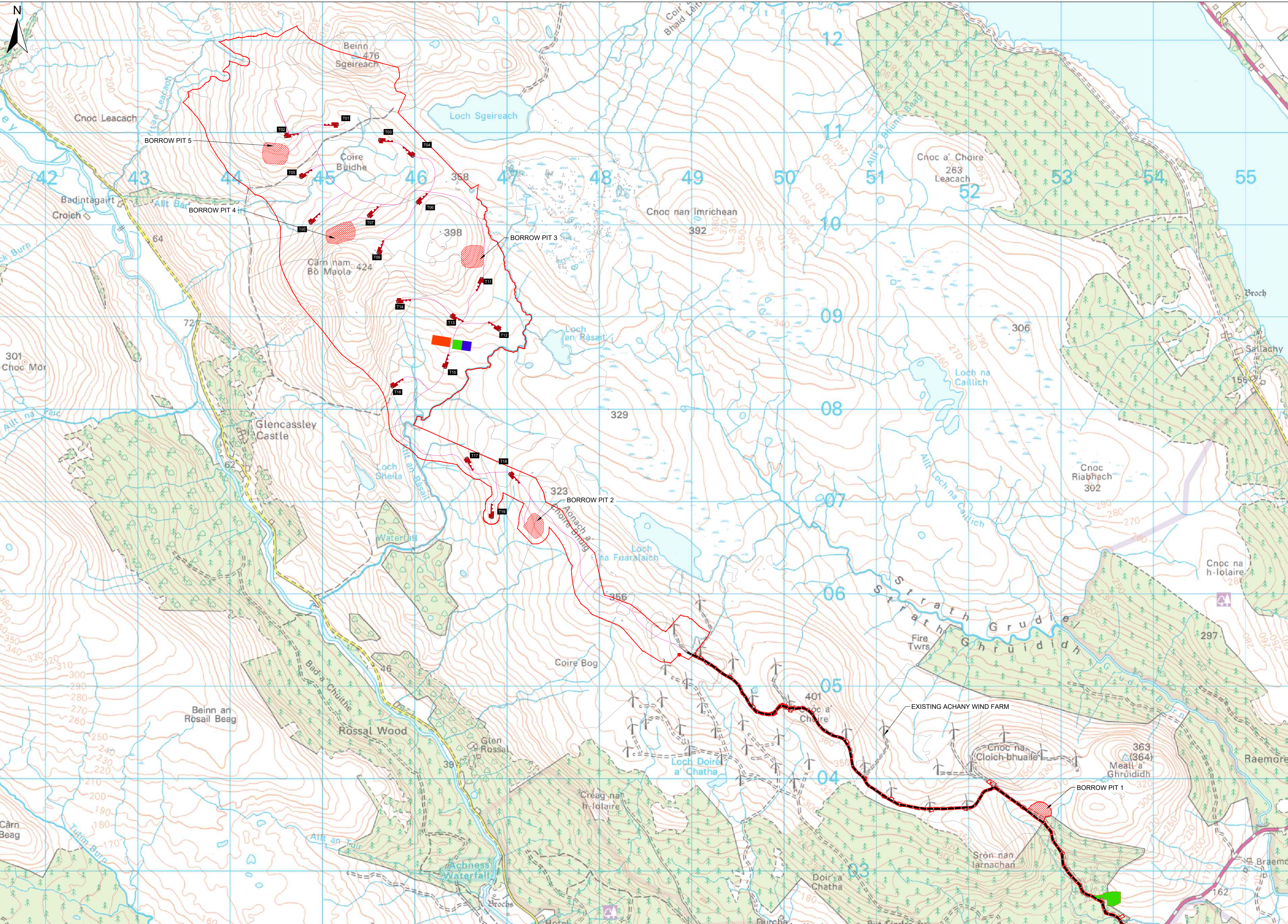
SITE LAYOUT SCALE 1:20000
