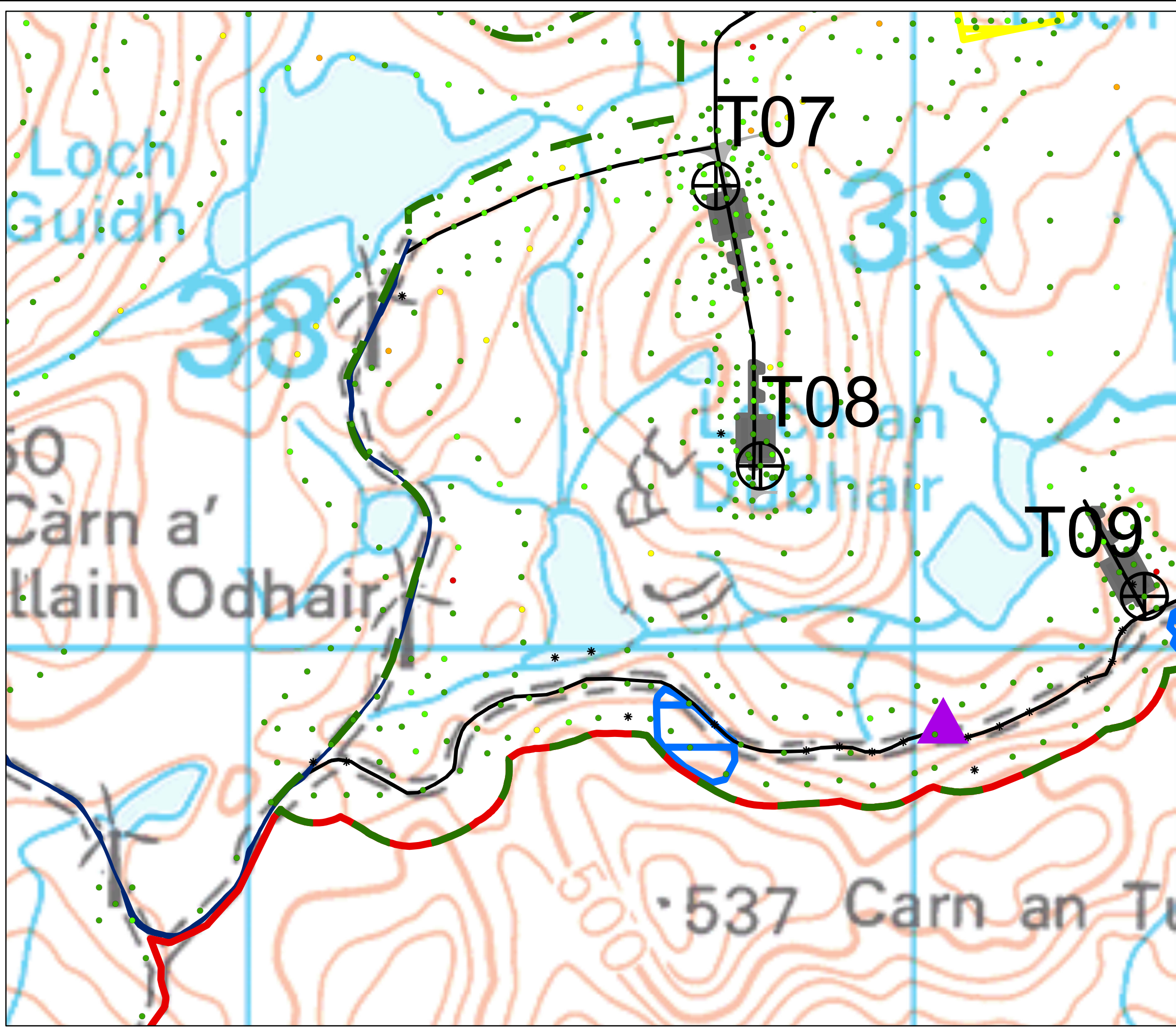
Figure 10.2 Page d Peat Depth Bhlaraidh Wind Farm Extension EIA Report
