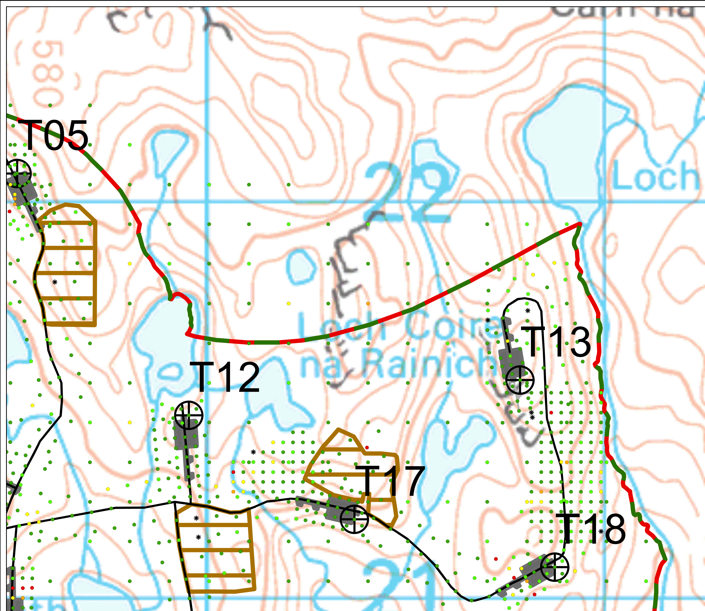
Figure 10.2 Page e Peat Depth Bhlaraidh Wind Farm Extension EIA Report
