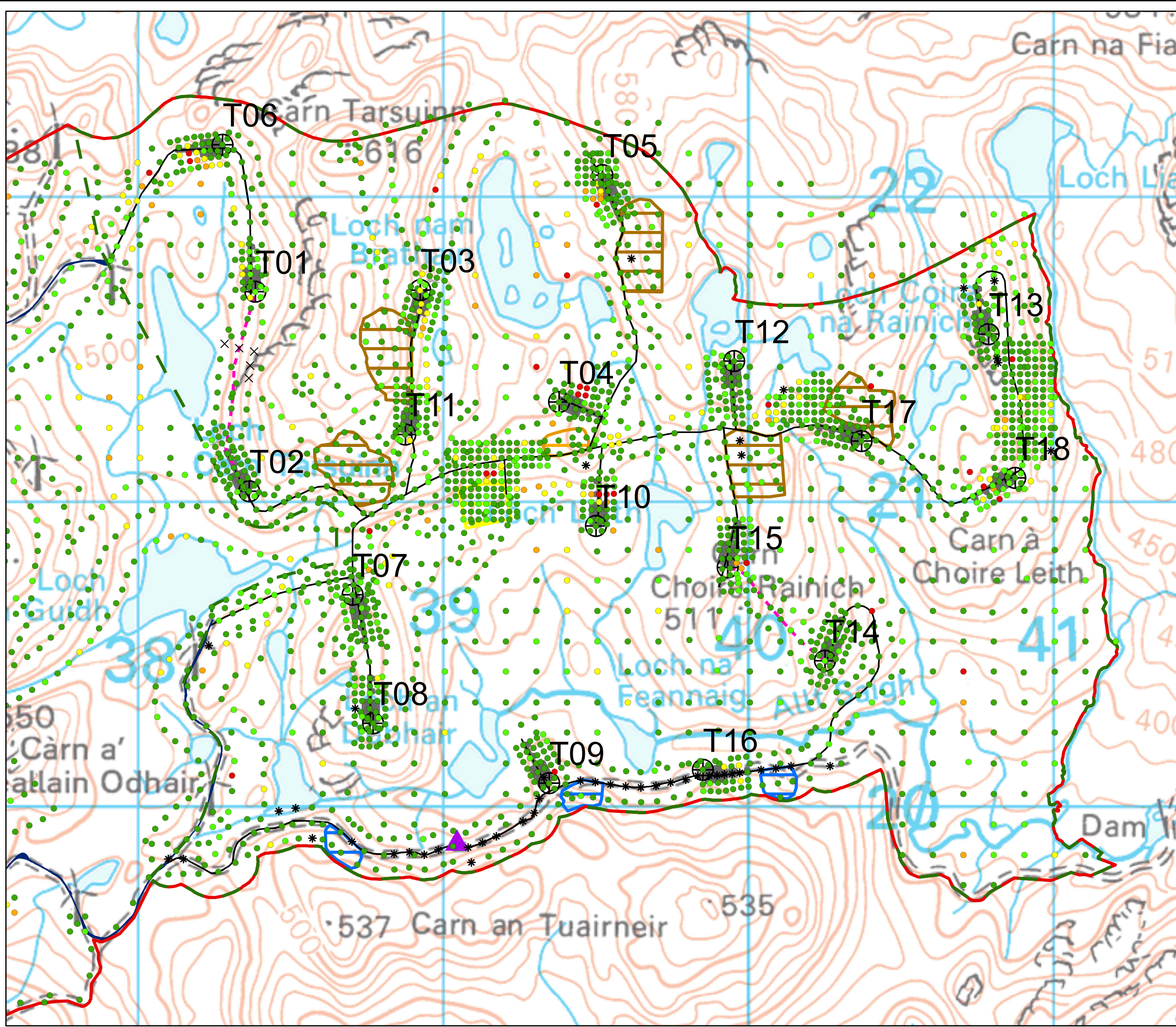
Figure 10.2 Page b Peat Depth Bhlaraidh Wind Farm Extension EIA Report
