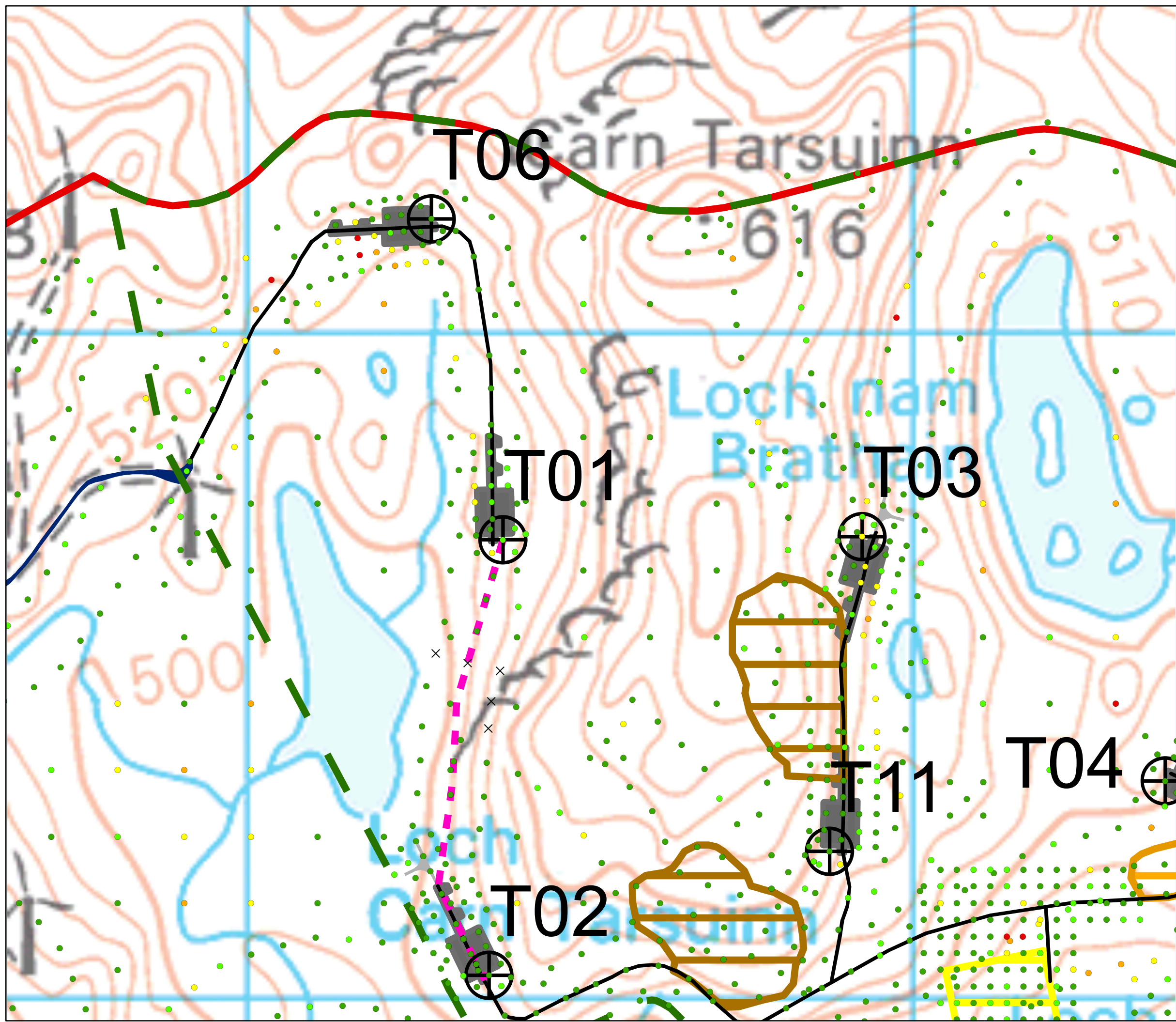
Figure 10.2 Page c Peat Depth Bhlaraidh Wind Farm Extension EIA Report
