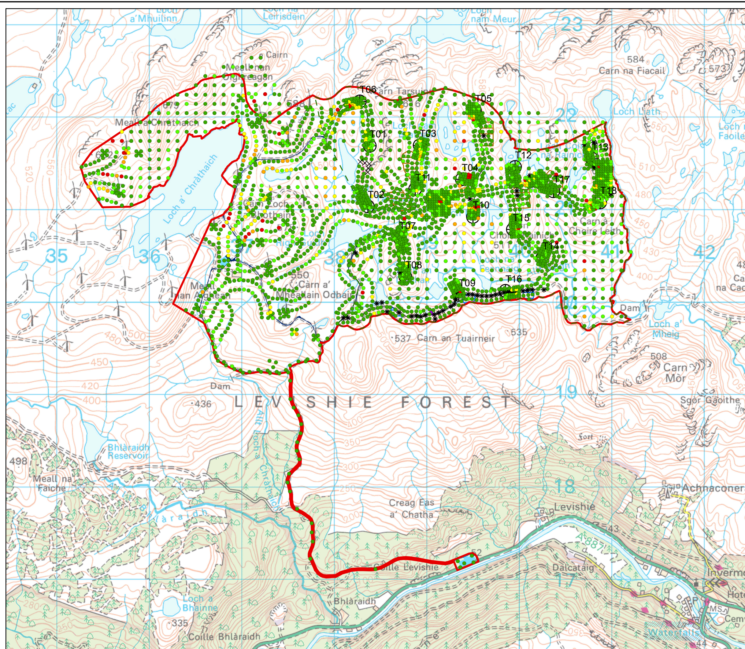
Figure 10.2 Page a Peat Depth Bhlaraidh Wind Farm Extension EIA Report
