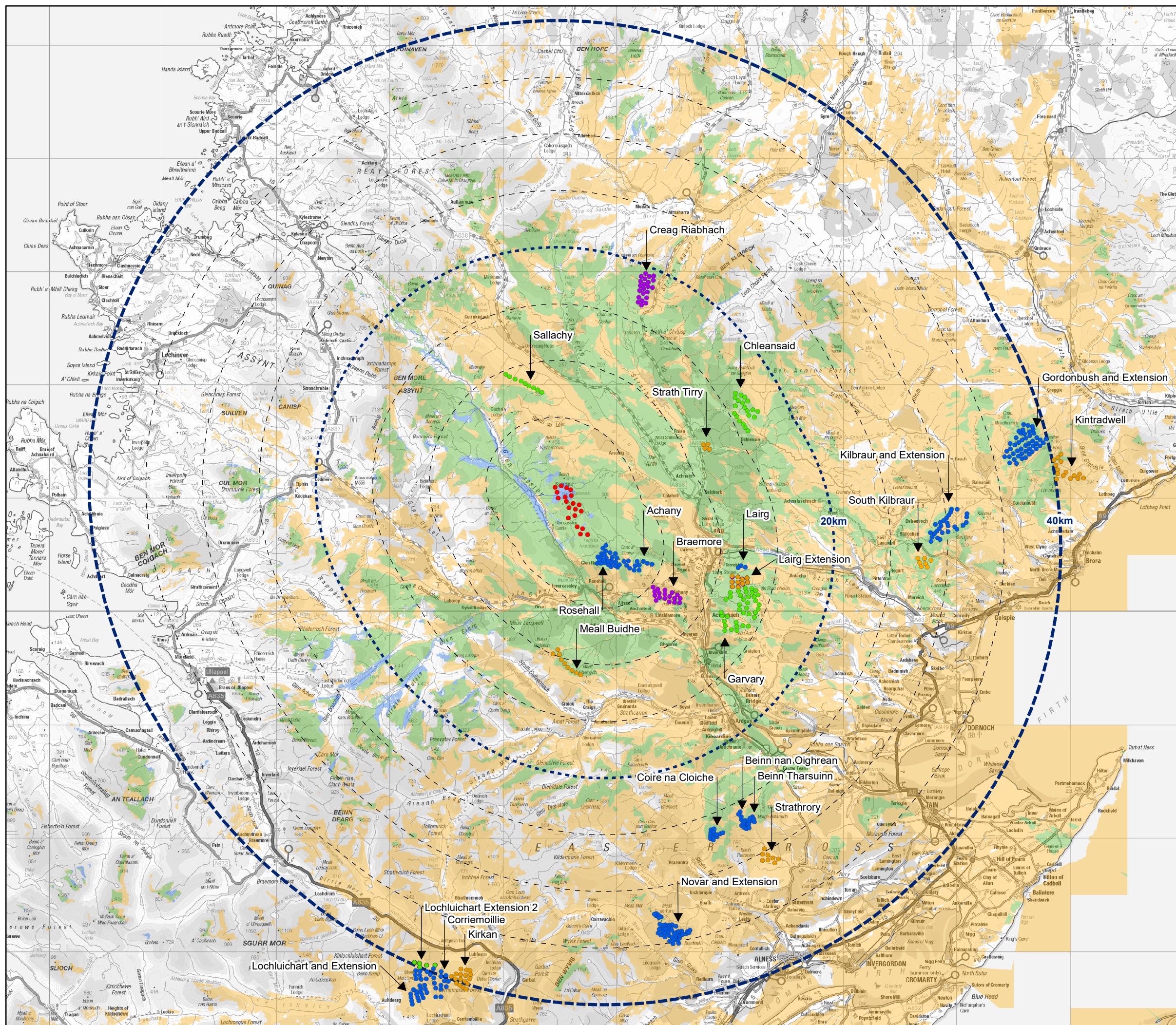
Figure 7.8.1 Cumulative ZTV - Proposed Development with All CLVIA Sites
