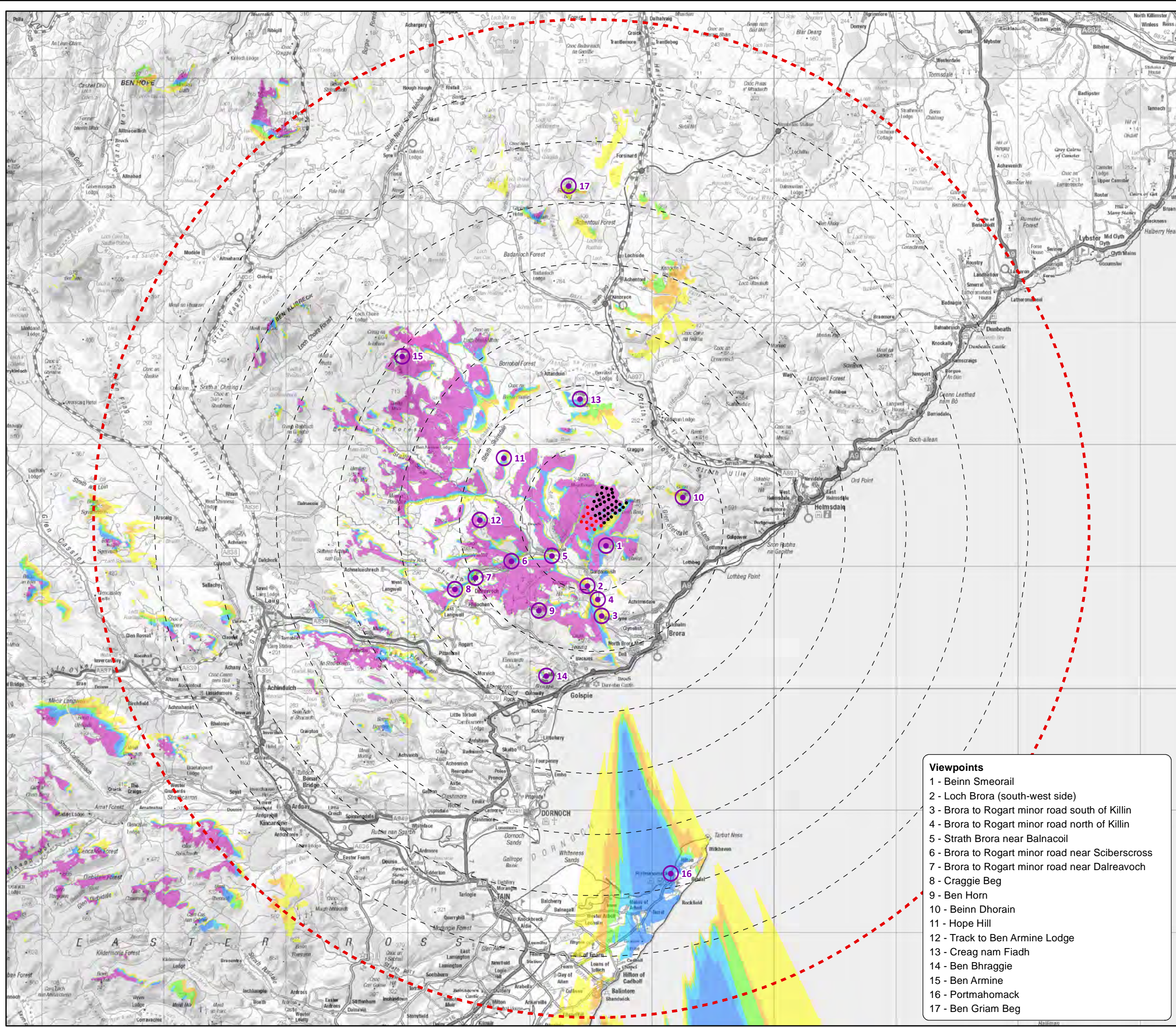
Figure 7.2a Hub Height ZTV with Viewpoints Gordonbush Extension Wind Farm EIA Report
