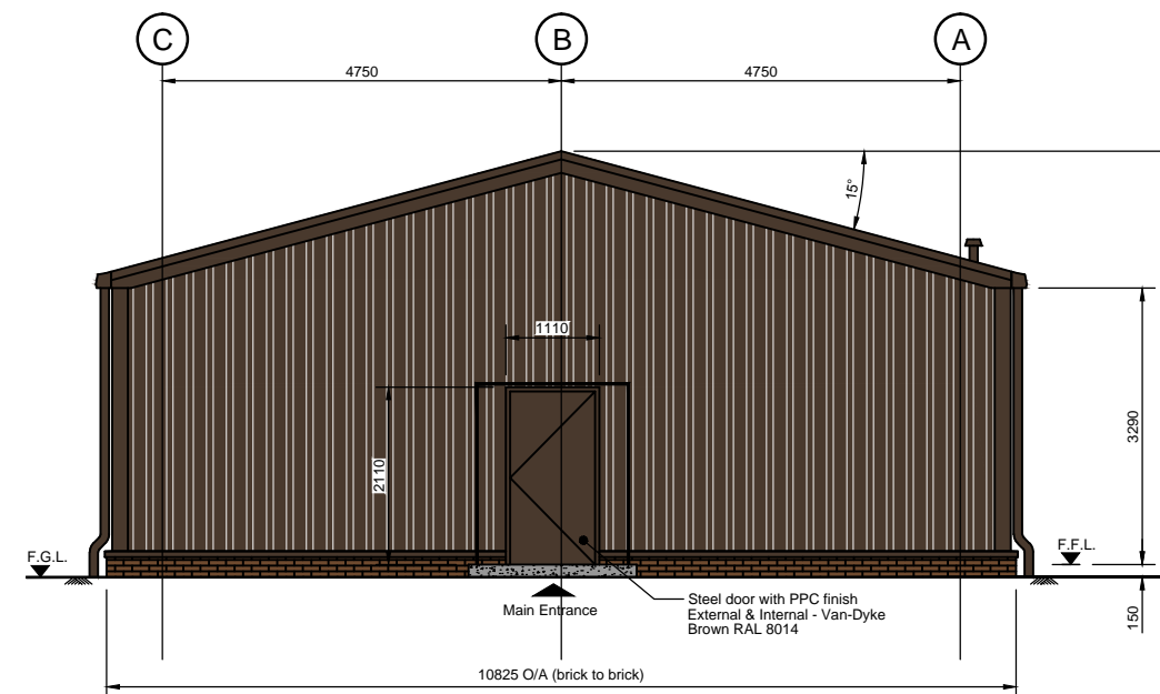
4 Gable Elevation Scale 1:100
