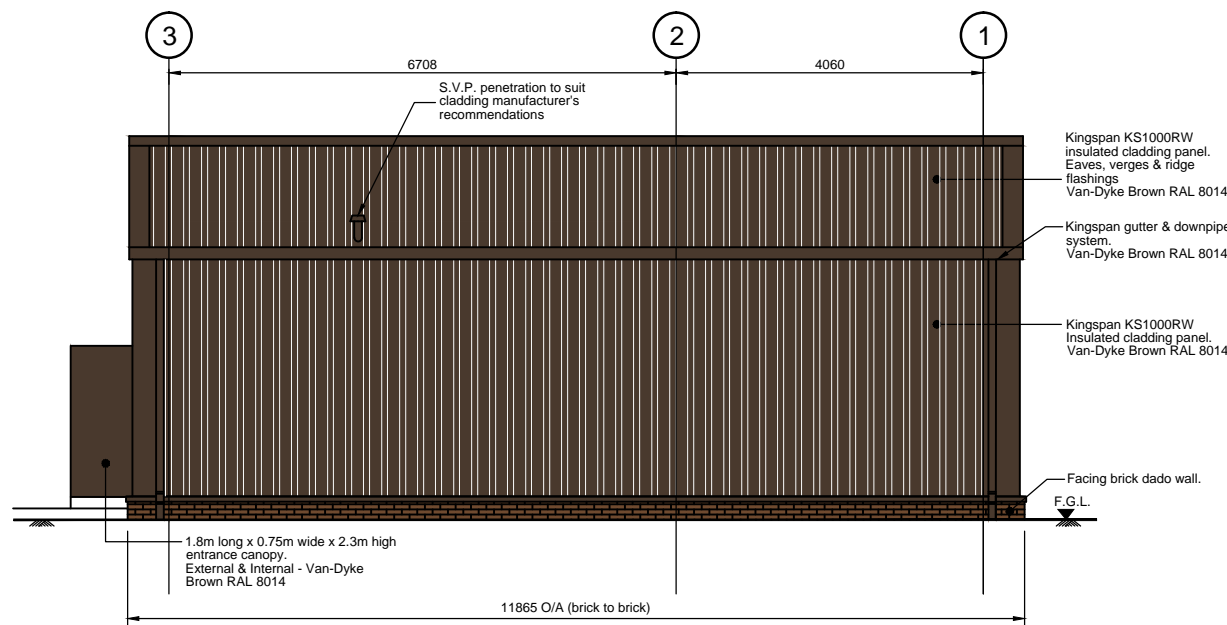
3 Rear Elevation Scale 1:100
