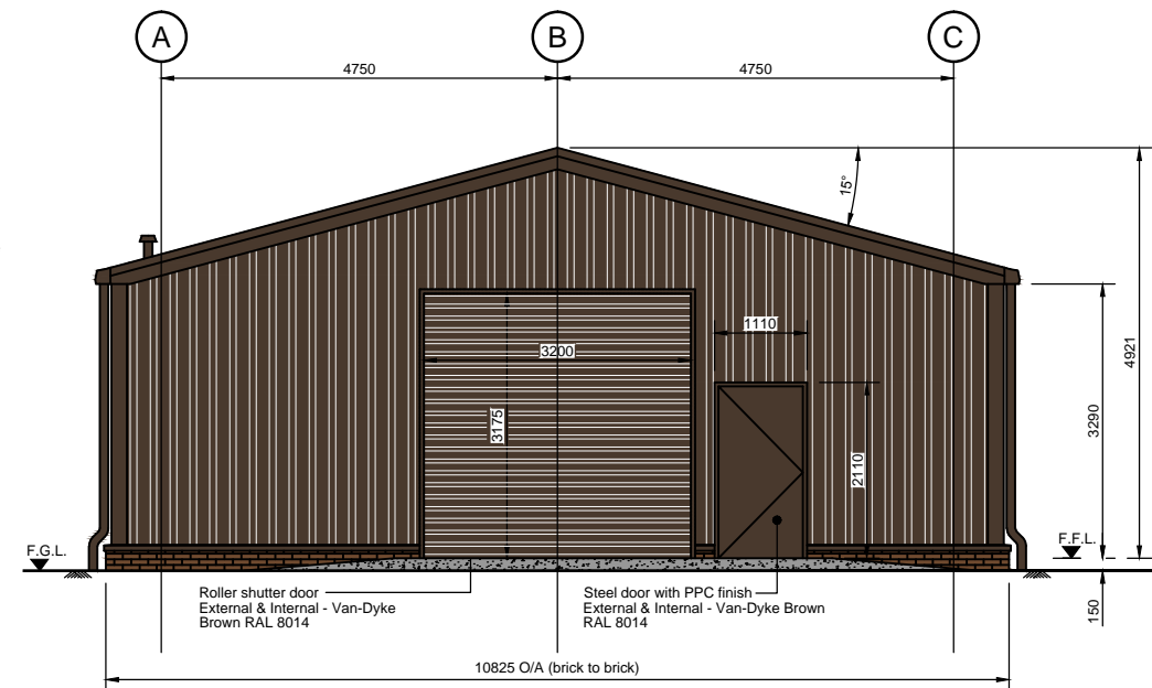
2 Gable Elevation Scale 1:100
