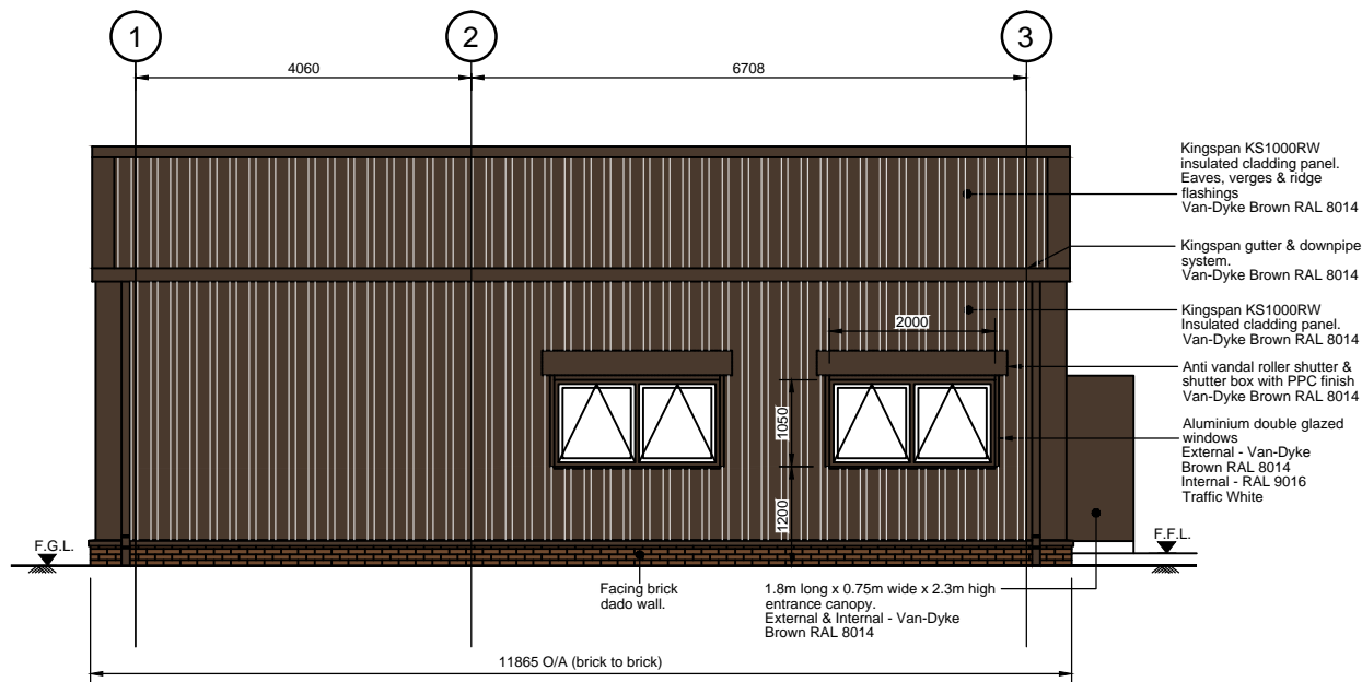
1 Front Elevation Scale 1:100
