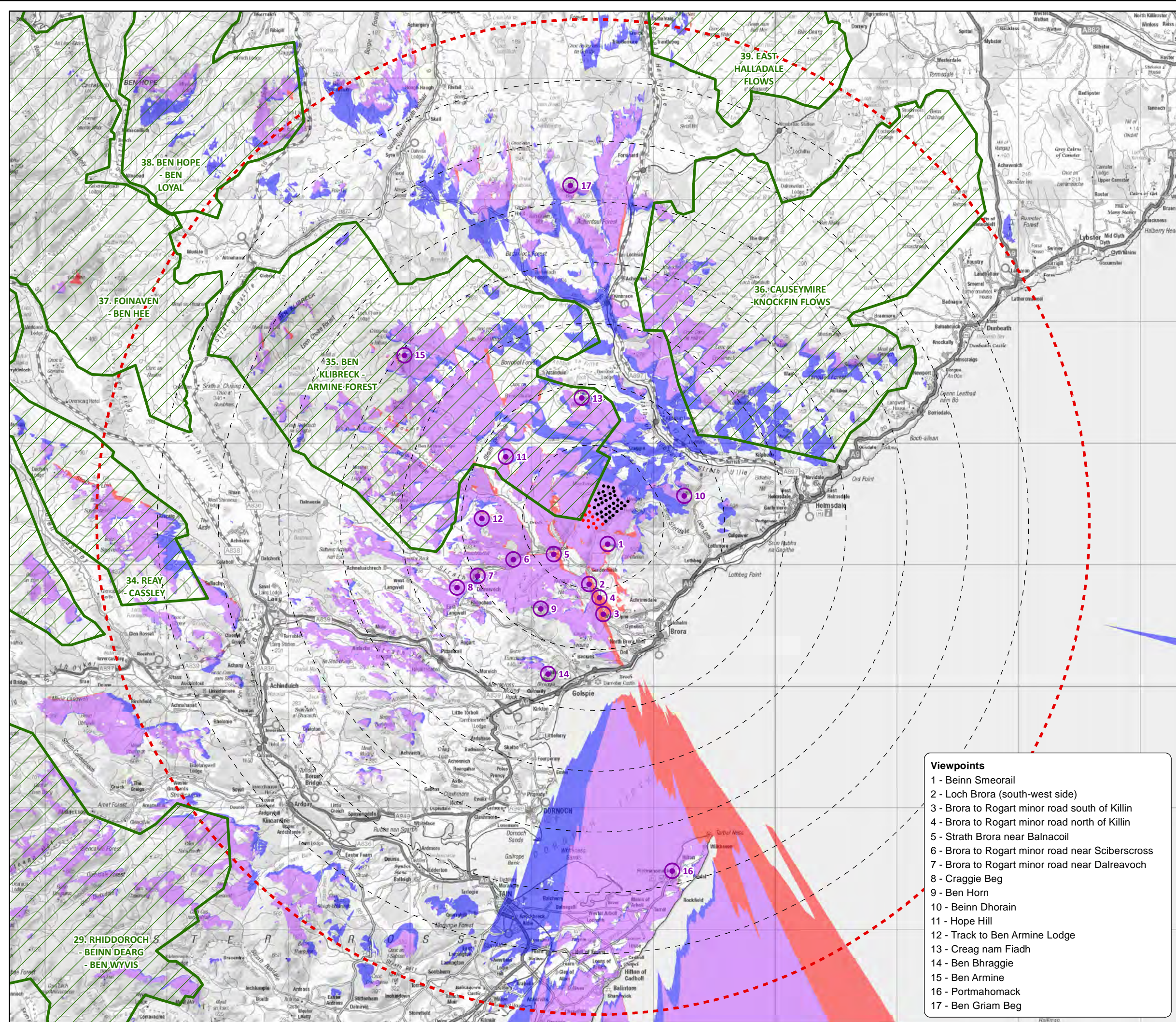
Figure 7.5c WLA and Comparative ZTV with Gordonbush Wind Farm Gordonbush Extension Wind Farm EIA Report
