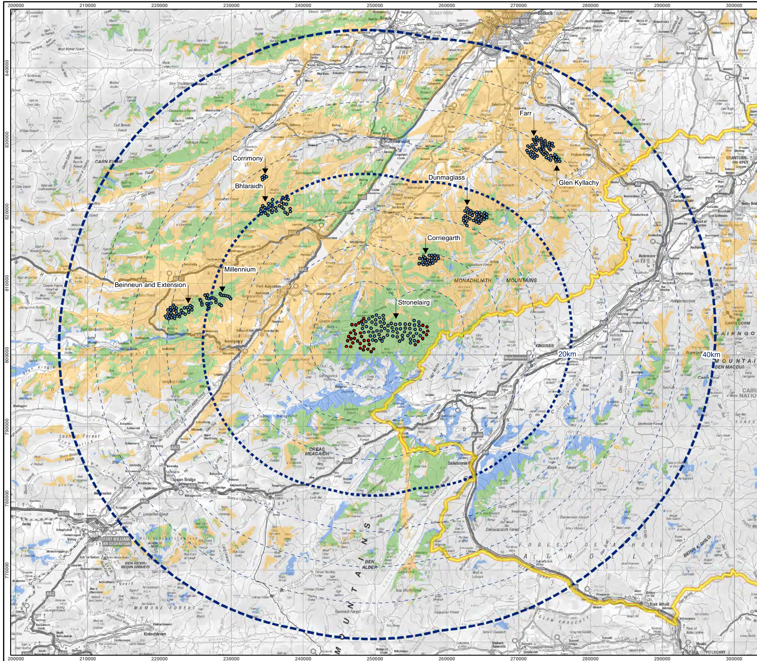
Figure 7.8.2 Cumulative ZTV - Proposed Development with Operational/Under Construction Sites Cloiche Wind Farm EIA Report
